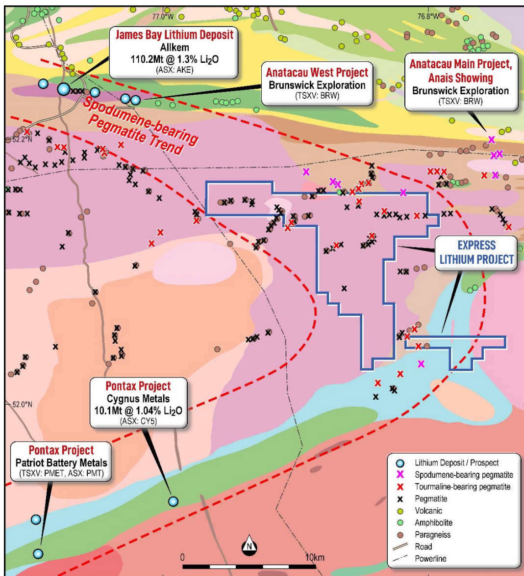
Figure 6: Express Lithium Project Boundary with Regional Geology Refer ASX Announcement of 15th March 2023 for full details of historically mapped pegmatites
