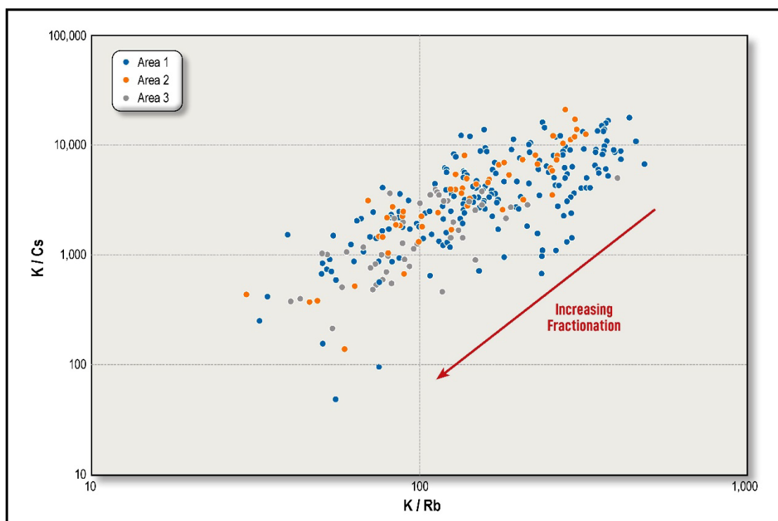
Figure 5: Plot of K/Cs vs K/Rb results for all Express samples showing fractionation of pegmatites.
