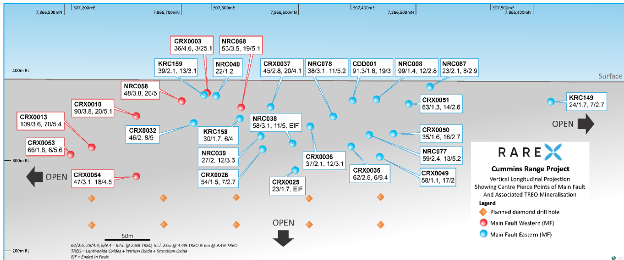
Figure 3. Vertical Longitudinal Projection showing centre points of Main Fault and associated TREO mineralisation
