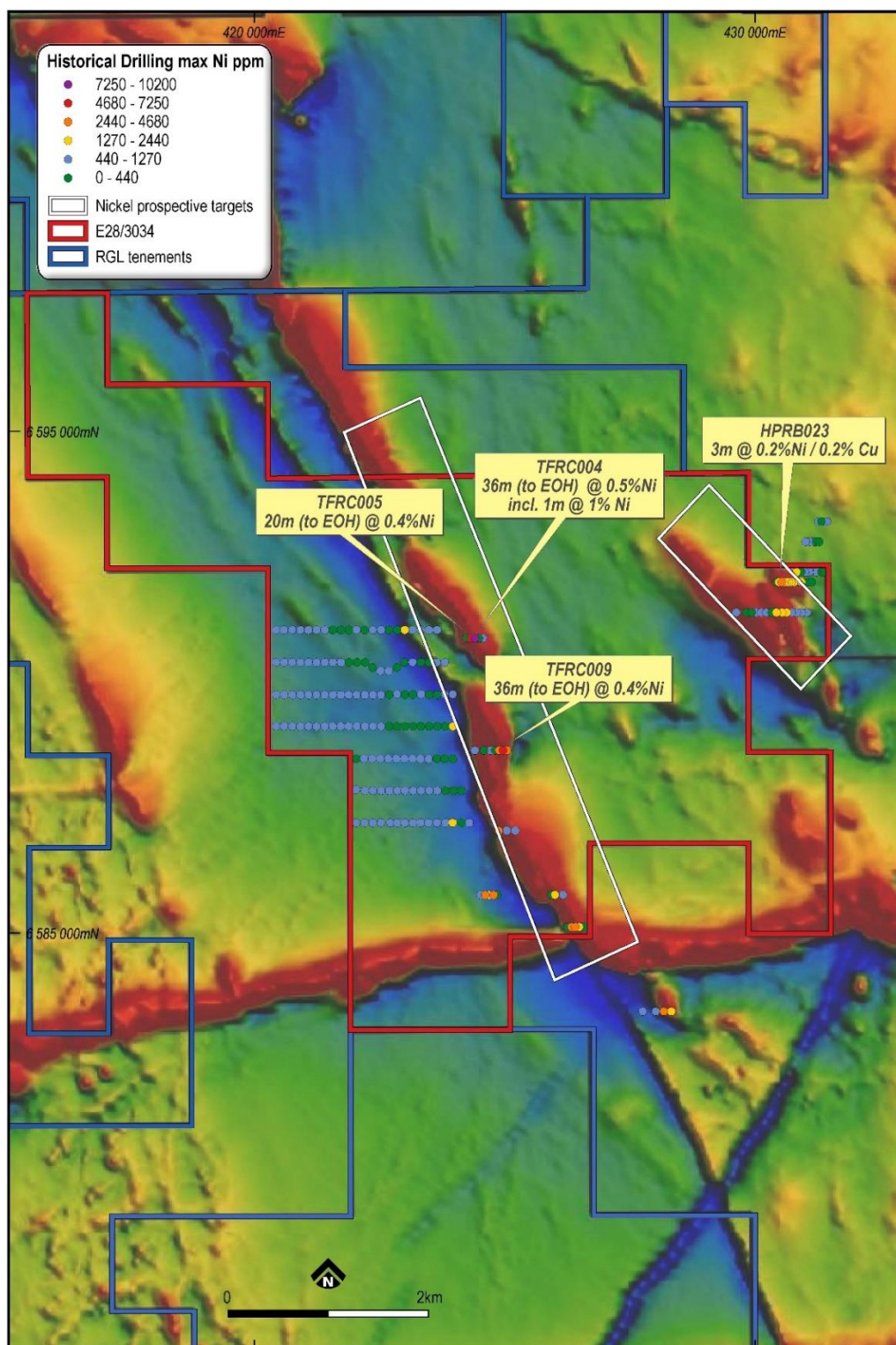
Figure 2: Geophysical image (TMI) of new tenement E28/3034 with historical drill collars and identified nickel prospectivity
