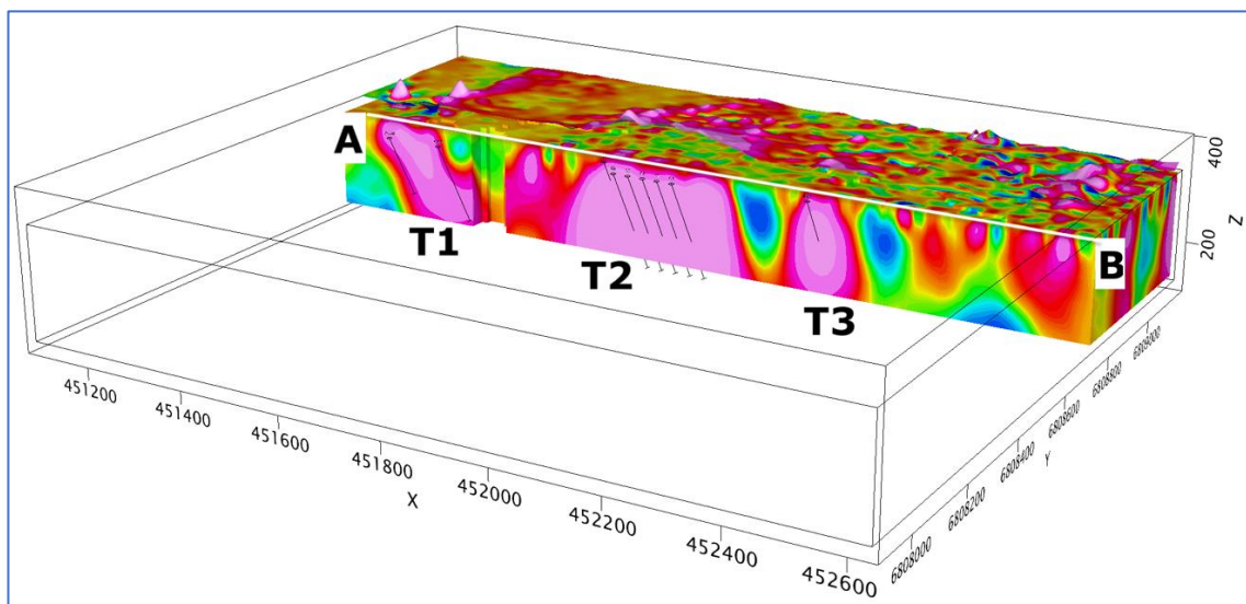
Figure 1: Ground magnetic results with sectional slice, confirm strong drill targets at T1 to T3 (See Figure 2 and Figure 3 for location information and Figure 3 with section line A-B) with 7 drill holes to a depth of ~250m-300m being designed for a 2,000m drill program.
