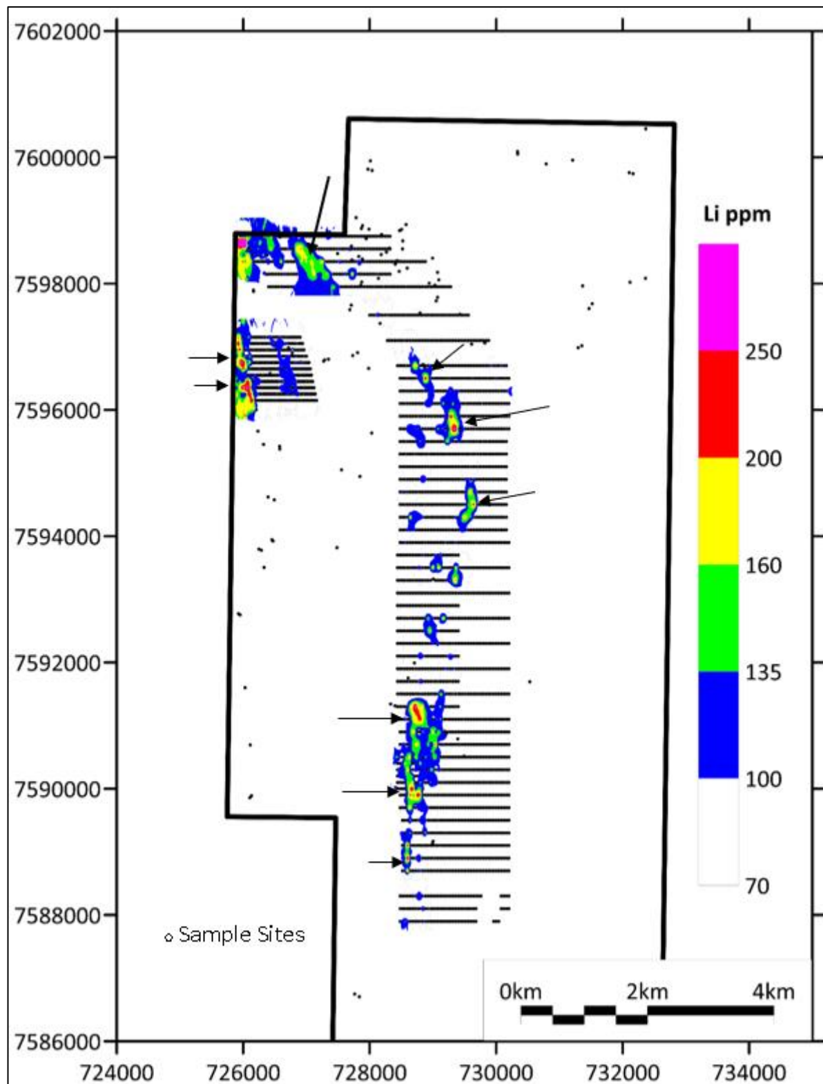
Figure 2: Tambourah Lithium (Li) geochemical results and sample locations of the 3,070-sample program, showing 9 new main targets.
