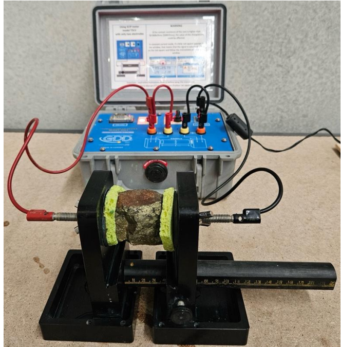
Figure 10: Prince Of Wales prospect sample RK008302 10.15% Cu and 65.8g/t Ag 11 , being tested for Induced Polarisation, chargeability, galvanic resistivity and inductive conductivity
