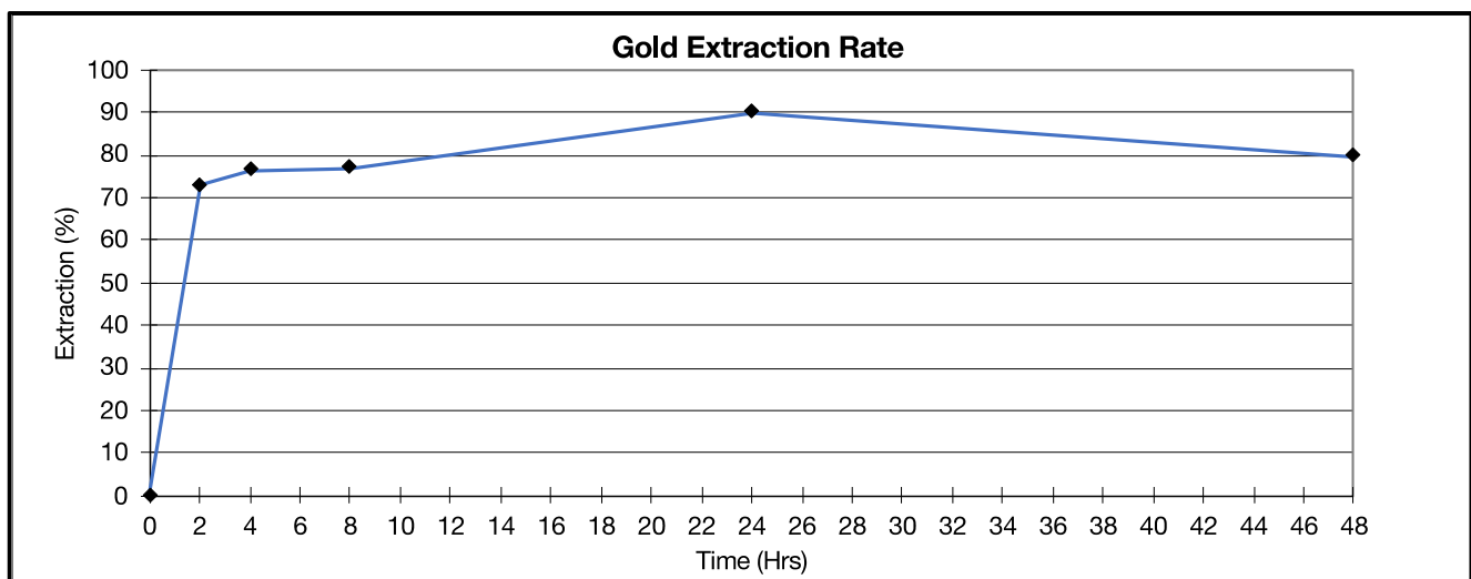
Figure 4: Leach Recovery Test Curve – Rougher Flotation Tailing
