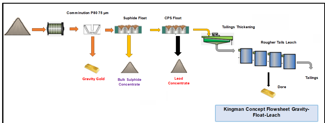
Figure 5: Gravity-Flotation-Leach Concept Flowsheet Tested
