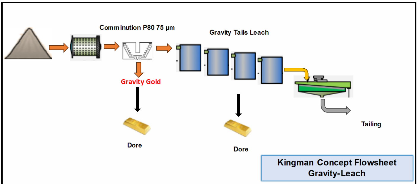
Figure 3: Gravity-Leach Flowsheet Tested
