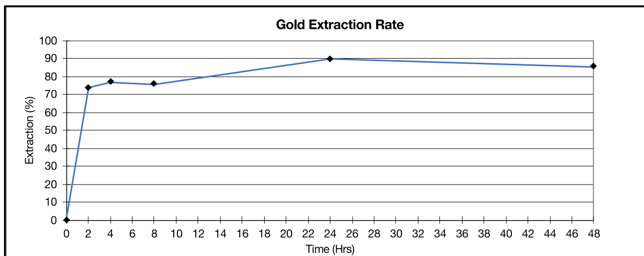
Figure 2: Leach Recovery Test Curve
