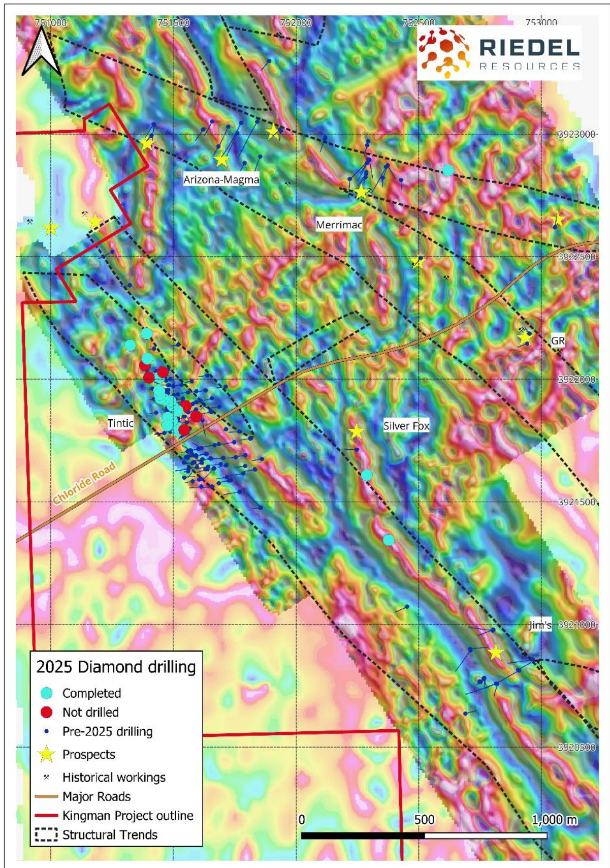
Figure 7: 2025 drill holes at Kingman Gold Project highlighting completed holes and planned holes not drilled overlain on aeromagnetic imagery (RTP-TILT_NEags).
