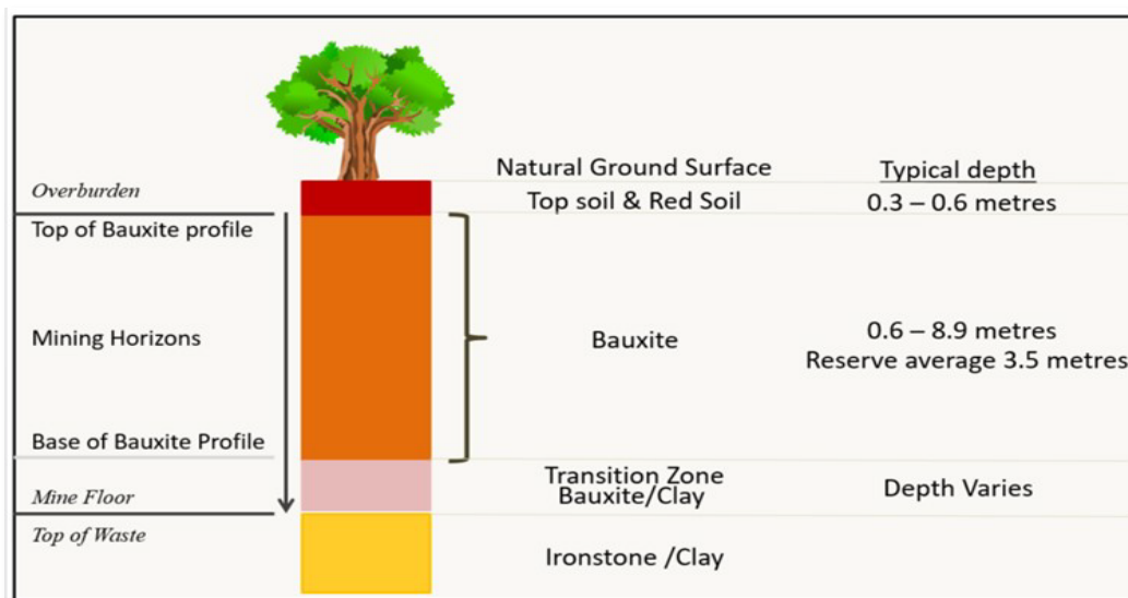
Figure 19 Type section - Amrun
