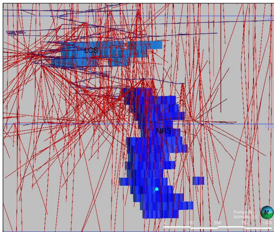
Figure 13 Oblique view of the LCS and NRS Ore Reserve stopes with drill holes in red. Grid is in Bingham Mine grid and in scale in feet – Kennecott Bingham Canyon underground
