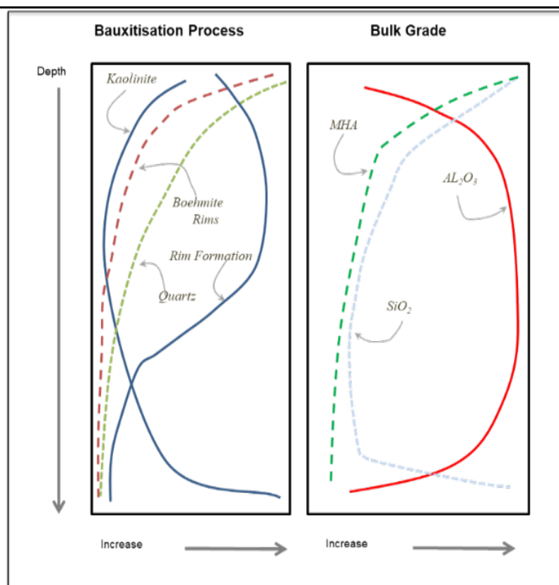
Figure 17 Relationships between the bauxite genetic processes and the resulting grade profiles - Amrun
