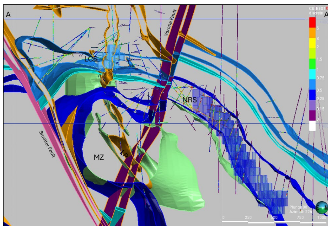
Figure 14 Typical cross section through the LCS and NRS deposits with the Ore Reserve stopes and geology. Section is 200 feet thick (61 m). Lower Commercial Limestone in light blue, Lower Lark Limestone in turquoise, Lower Jordan Limestone in dark blue, Monzonite (MZ) in green, and Latite Porphyry Dikes in Orange. Holes are coloured by assayed copper grades. LCS and NRS areas labelled. Grid is in Bingham Mine grid and in scale in feet. Section location is denoted in Figure 11 and Figure 12 – Kennecott Bingham Canyon underground
