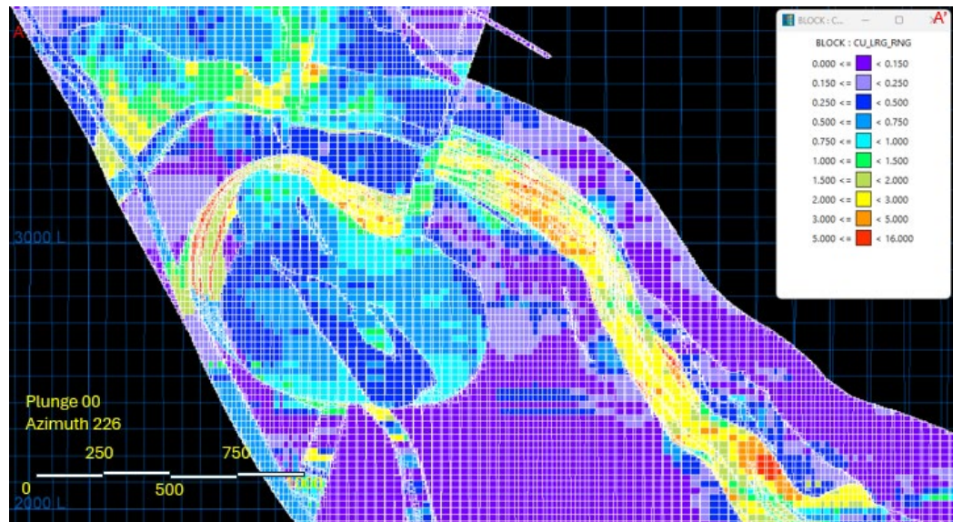
Figure 15 Typical cross section through the LCS and NRS deposits showing estimated copper distribution within the skarn beds. Grid is in Bingham Mine grid and in scale in feet. Section location is denoted in Figure 11 and Figure 12 – Kennecott Bingham Canyon underground
