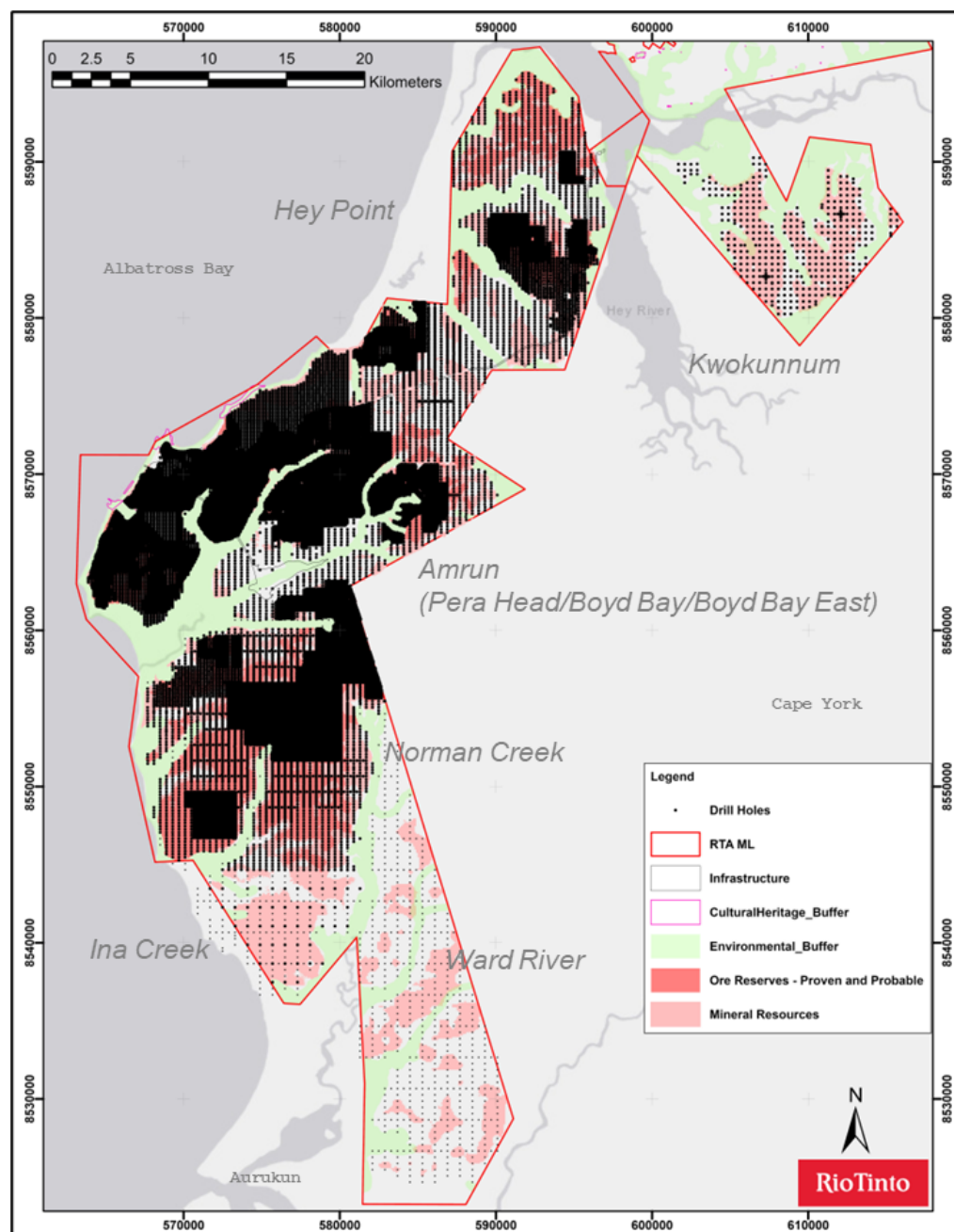
Figure 18 Current drill hole plan map - Amrun
