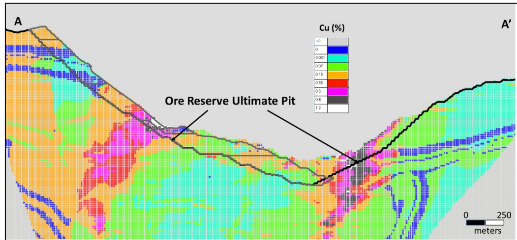
Figure 10 Cross section A-A' through the Bingham Canyon orebody showing copper mineralisation – Kennecott Bingham Canyon open pit
