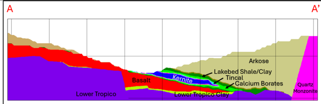
Figure 24 Cross section showing the geological resource model and rocktype domains - Boron
