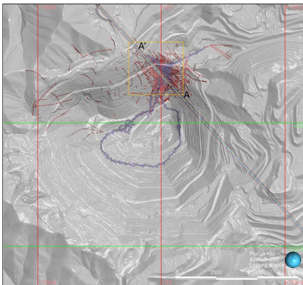
Figure 11 Drill holes used for the LCS and NRS Mineral Resource estimation, in red, in relation to the Bingham Canyon open pit in gray. Current underground workings in purple. Location of Figure 12 in orange. Location of cross sections A'-A. Grid is in Bingham Mine grid and in scale in feet – Kennecott Bingham Canyon underground
