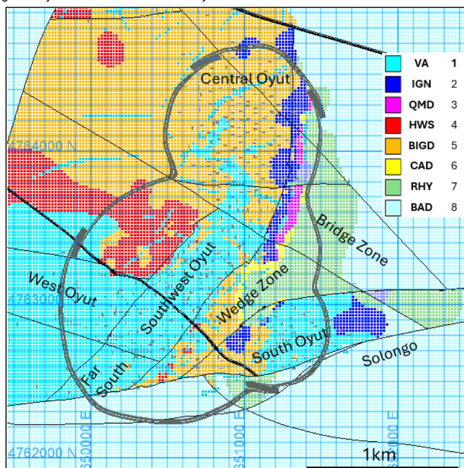
Figure 7 Plan section at 1000 m elevation showing geological model of the Oyut deposit including drill holes (grey) and fault blocks (black) – Oyu Tolgoi
