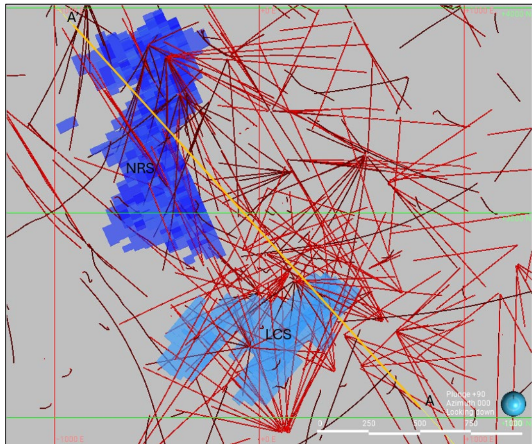
Figure 12 Plan view of the drill holes used for the LCS and NRS Mineral Resource model in red. NRS Ore Reserve stopes in dark blue and LCS Ore Reserve stopes light blue. Location of cross sections A'-A in orange. Grid is in Bingham Mine grid and in scale in feet – Kennecott Bingham Canyon underground
