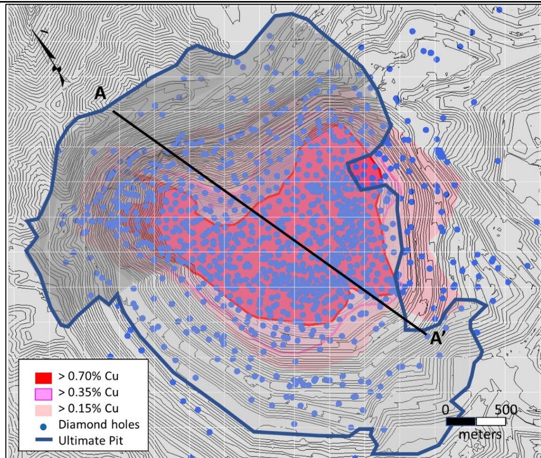
Figure 8 Current pit drill hole intersections including those contained within the Ore Reserve pit – Kennecott Bingham Canyon open pit
