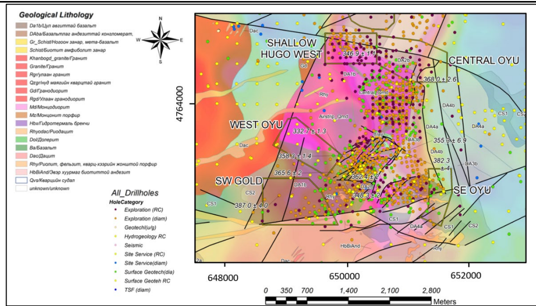
Figure 6 Plan view showing drill hole collar locations and geology of the Oyut deposit – Oyut Tolgoi
