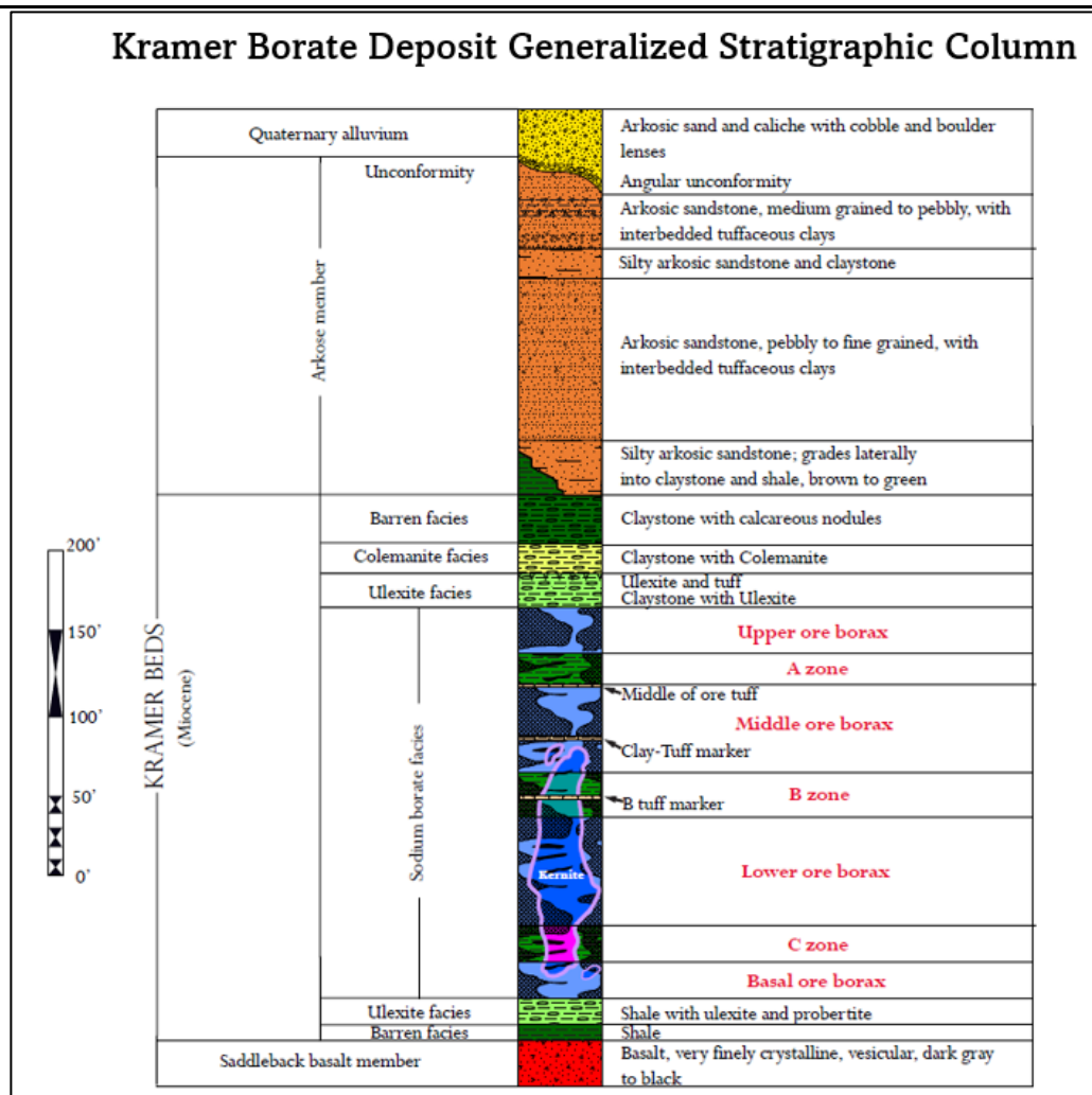
Figure 21 2024 Stratigraphic column of the Kramer deposit - Boron
