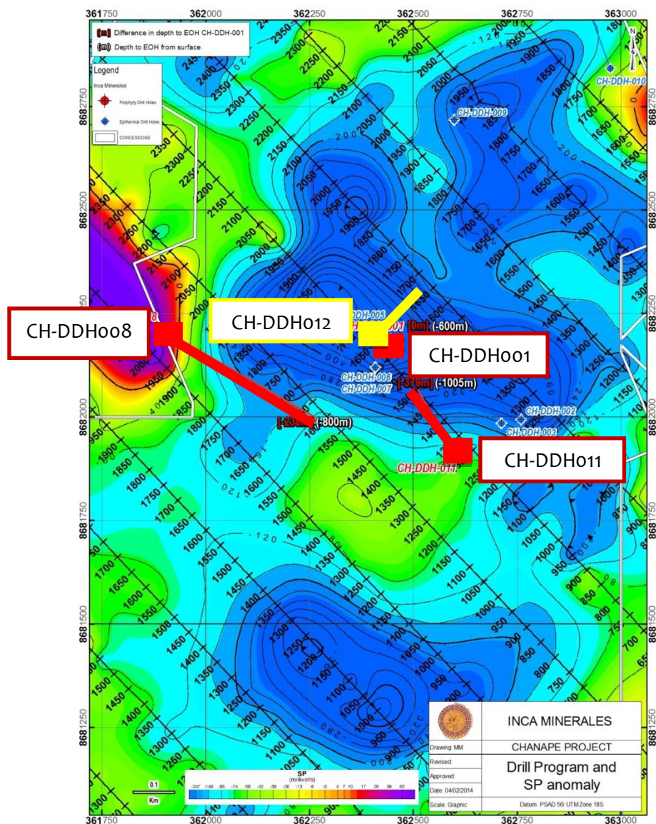
Figure 1: Drill hole location plan of all deep holes, including CH-DDH012 (the current hole), CH-DDH001 (the “discovery hole”), CH-DDH008 and CH-DDH011. The figure shows their relative position to that of a large SP Anomaly (marked in blue).
