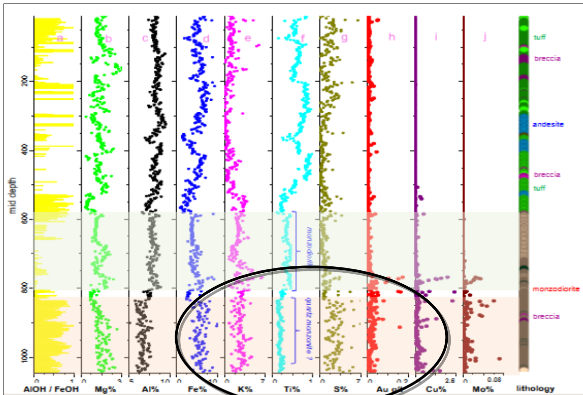
Figure 3: Hydrothermal alteration in comparison with geochemistry. Of particular note is the distinction made between an upper (and earlier) monzodiorite and a lower (later) mineralising quartz-monzonite. It is the latter that is more closely related to the porphyry mineralisation .
