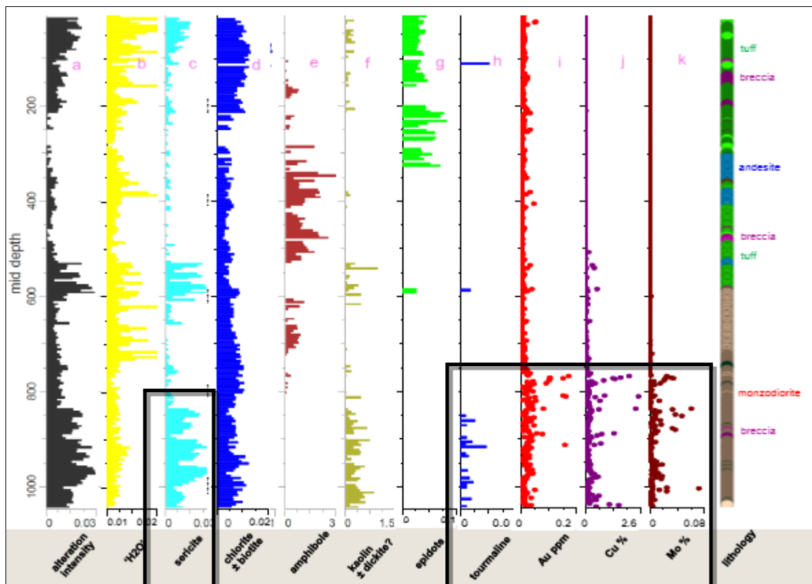
Figure 2: Hydrothermal alteration in comparison with mineralisation. Three distinct zones of alteration are recognised, the deepest corresponding to logged monzodiorite hosts porphyry style mineralisation. Refer to Figure 3 for further comment.
