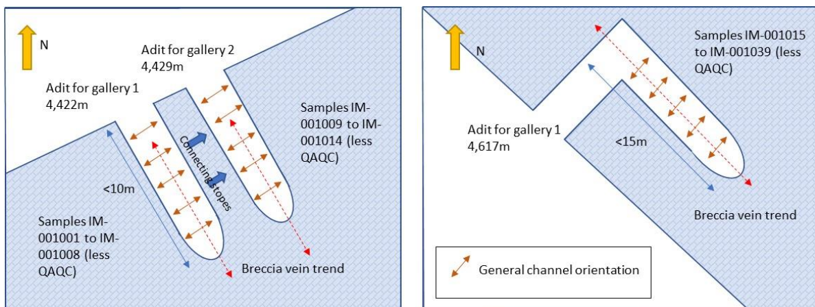
Figure 8: Schematic plans of Vilcapuquio (left), Torrepatá (right)
