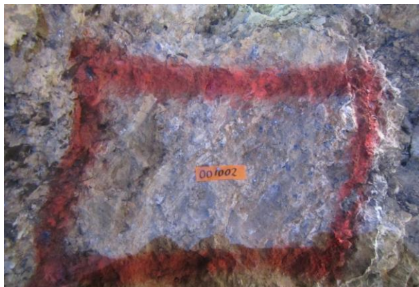
Figure 2: ABOVE LEFT Photo of channel sample IM-001002 containing 23.55% Zn, 10.3g/t Ag, 12.38% Pb . The sample contains visible smithsonite and galena as matrix material within a breccia vein. ABOVE RIGHT Photo of channel sample IM-001008 containing 18.57% Zn, 19.86% Pb . The sample is significantly more weathered (more Fe-oxides) than IM-001002. The brown colouring of IM-001008 is similar to previous samples that are equally weathered which contain very high levels of Zn (Refer to Figure 3).
