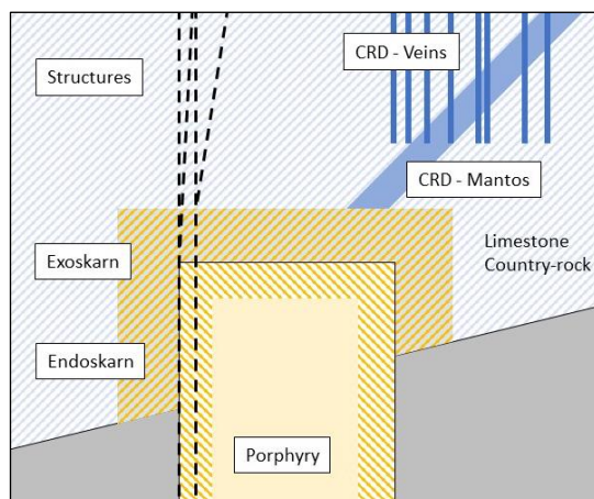
Figure 4 LEFT: A simplified schematic porphyry model showing the juxtaposition of porphyry deposits, skarn deposits (exo = outside the porphyry along the contact, endo = inside the porphyry along the contact), structure-related deposits and manto and vein carbonate replacement deposits (CRD's). The broad elements of this model are known at Riqueza and its surrounds: mineralised porphyries intrusions, skarn mineralisation, mineralised structures, mantos and veins within a limestone country-rock setting.
