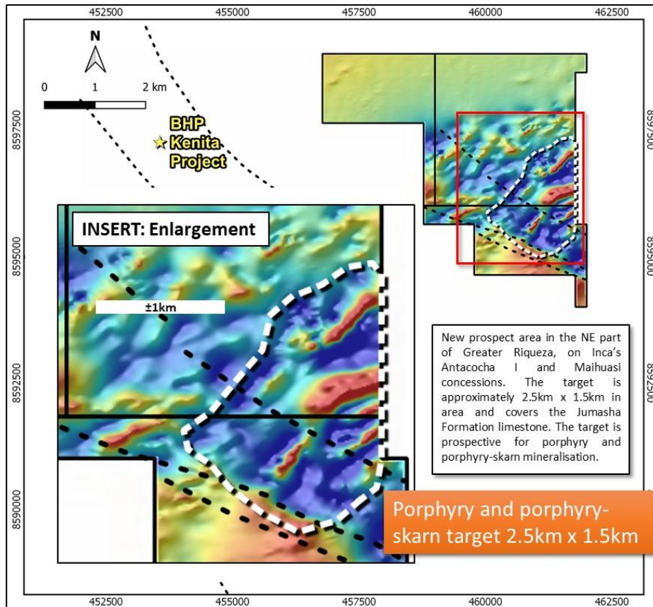
Figure 3 LEFT: A preliminary TMIRTP image showing raw, gridded total magnetic intensity data reduced to pole providing a basic level of interpretation. Highlighted is the Yanacolipa porphyry and porphyry-skarn target-centre
