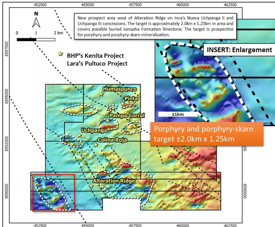
Figure 1 LEFT : A preliminary TMIRTP image showing raw, gridded total magnetic intensity data reduced to pole providing a basic level of interpretation. Highlighted is the Tayapampa porphyry and porphyry-skarn target-centre.
