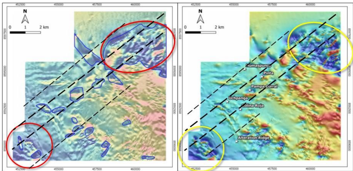
Figure 1 ABOVE LEFT: TMIRTP over TMIRTP-1VDAGC image highlighting two large areas of reversely magnetised anomalies of the SW Corner and NE Area (red circles). The two areas are located on the transfer zone, discussed in previous ASX announcements. ABOVE RIGHT: TMIRTP image showing the similar magnetic expression (yellow circles) of both areas. Large reversely magnetised anomalies (areas of blue patternation) are interpreted to be caused by intrusive and hydrothermal event(s) during periods of opposite magnetic polarity such as that occurring during the Miocene period – a geological time during which many of the Peru porphyry belt mineralised intrusive events occurred.
