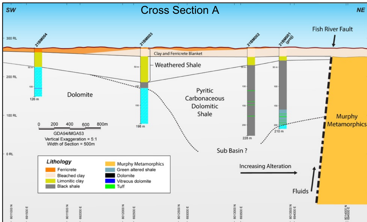
Figure 7 Cross Section A
