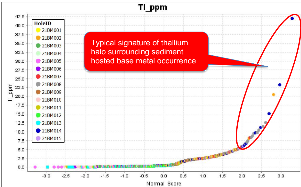
Figure 5 Thallium (TI) results coloured by RC drillhole. Note holes 21BM001, 21BM002, 21BM007, 21BM008, 21BM014 and 21BM015 intersected thick carbonaceous siltstone and shale units.
