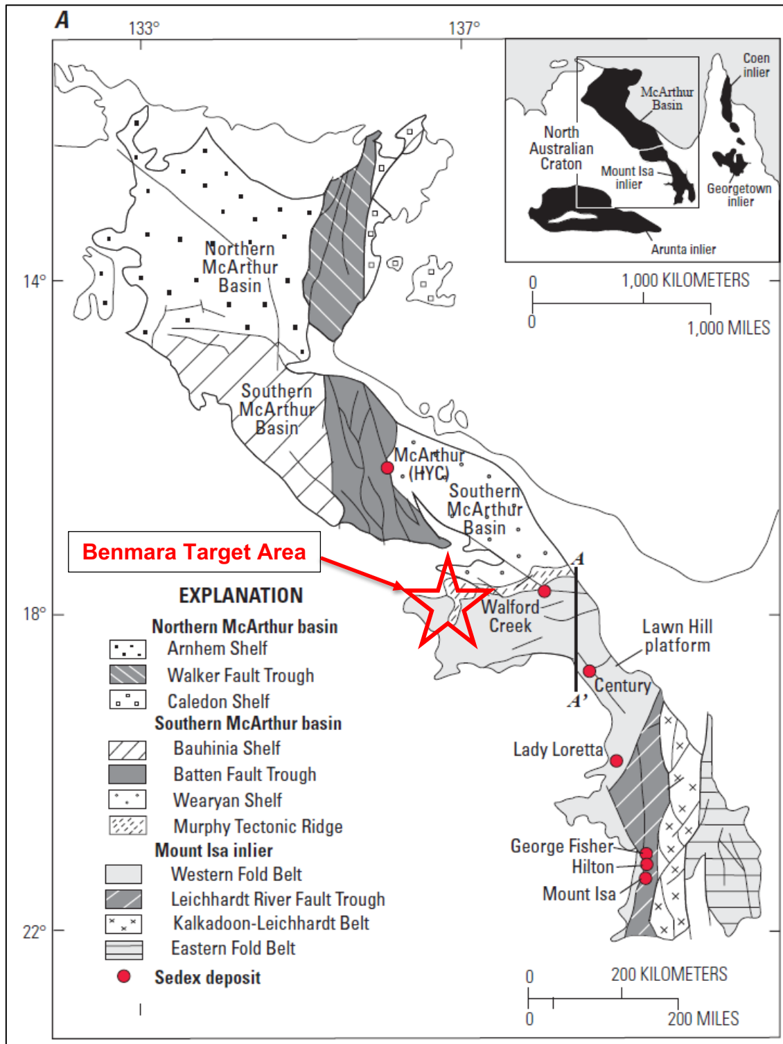
Figure 10: Geology of the Mt. Isa-McArthur basins of northern Australia showing the location of major tectonic elements and the position of SEDEX deposits (Emsbo et al, 2016).
