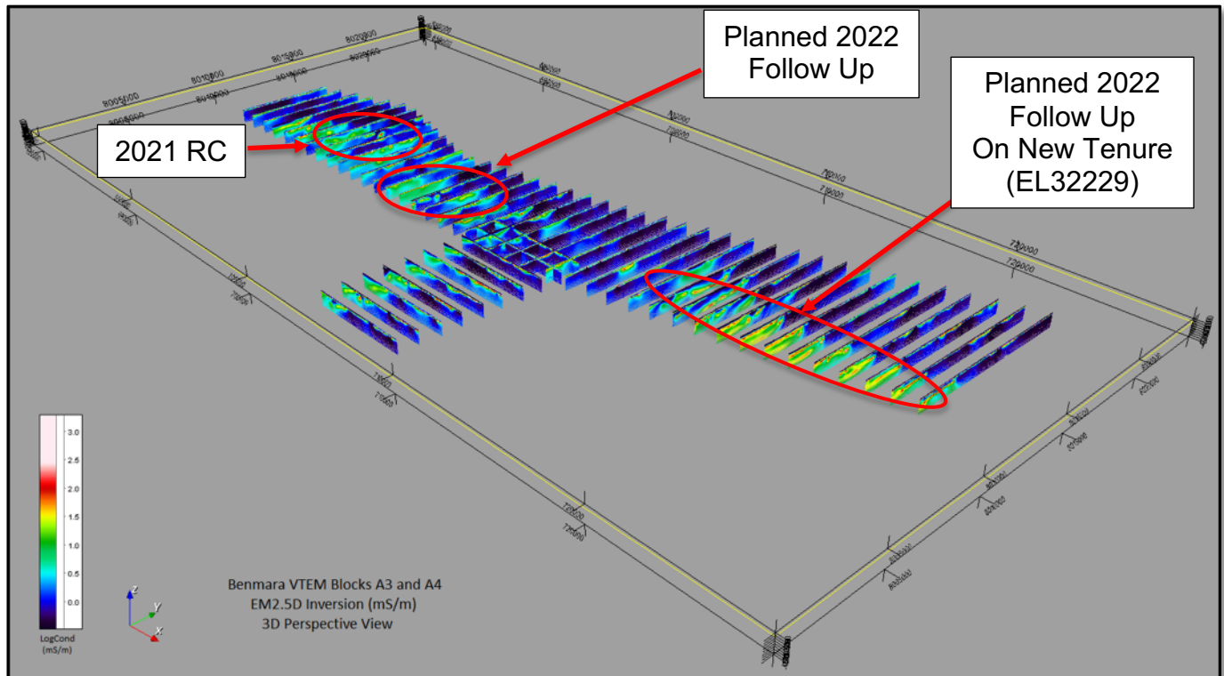
Figure 9 - 3D perspective view looking north-west on the Benmara 2.5D Inversion. 2021 RC location relative to planned 2022 drilling areas
