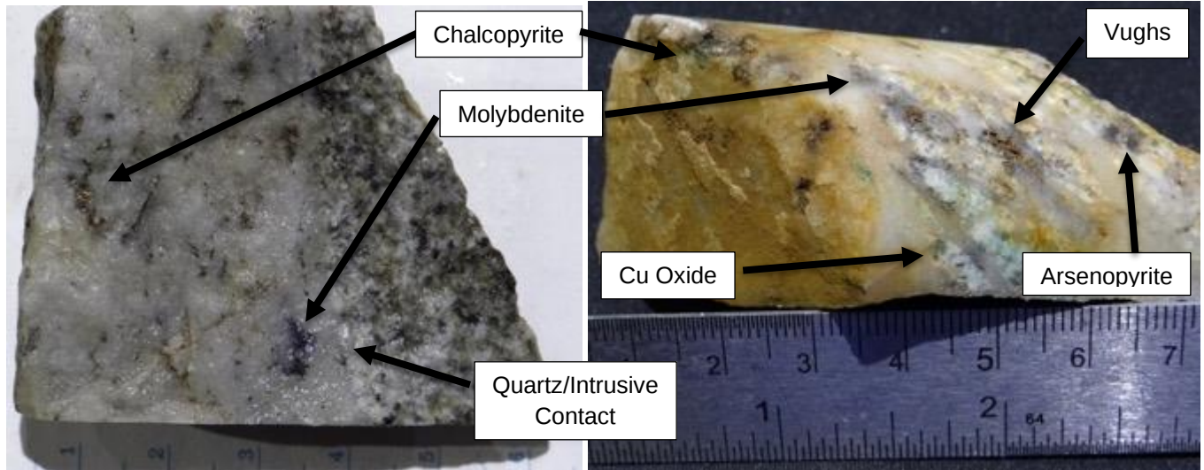
Figure 3 Elaine Prospect, HoleID 00ED-01, (left) 61.97m depth, > 3cm thick quartz vein cross cutting altered (propylitic?) biotite \pm hornblende quartz monzonite porphyry with visible chalcopyrite and molybdenite (B Vein) and (right) 71.7m depth, > 3cm quartz vein cross cutting quartz monzonite porphyry with chalcopyrite, molybdenite, arsenopyrite, Cu oxides and oxide filled vughs after sulphides (B Vein).
