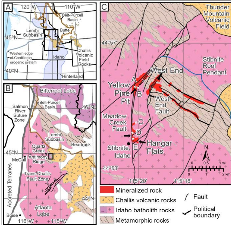
Figure 12: Location plan, regional geology and local geology of the Stibnite-Yellow Pine deposits. This figure is copied and unmodified from N. E. Wintzer (2019) 5 . The key purpose for the inclusion of this figure in this announcement is to illustrate the project-scale juxtaposition of mineralisation, faults/shares and the intrusive rocks (pink) and the intruded rocks (pale brown). The local geological setting of the Stibnite-Yellow Pine deposit area is very similar to the Horse Heaven Project area.
