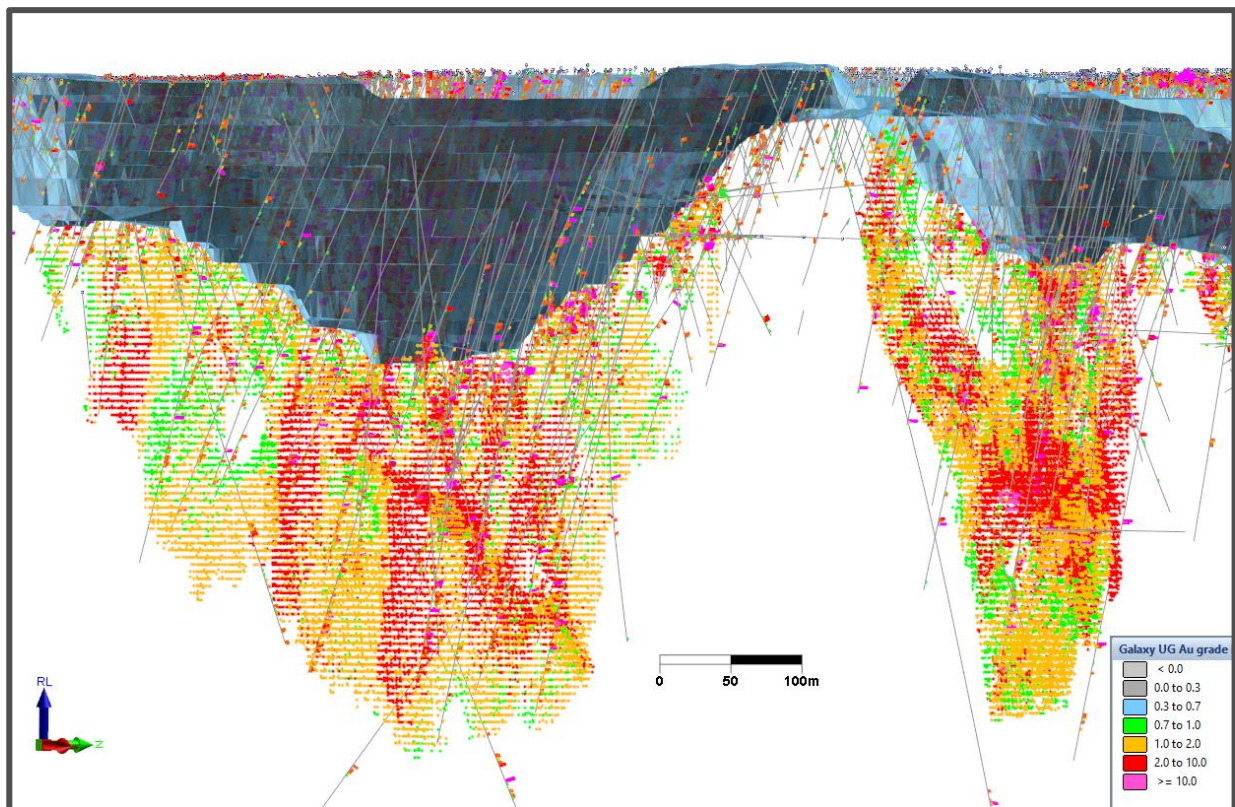
Figure 4: Galaxy Underground BIF Drilling & Model – 3D view to NW
