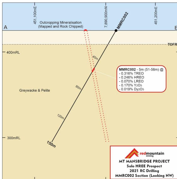
Figure 2 – MMRC002 Cross-Section
