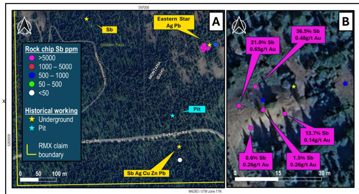
Figure 2: (A) Google Earth image of the southwest corner of Red Mountain's Thompson Falls Project Area showing the location of historical mines and antimony rock chip sample results from the initial sampling. (B) Detail over the Eastern Star area, showing analytical results for Sb and Au for samples containing over 0.5% (5000ppm) Sb and 0.1ppm Au.
