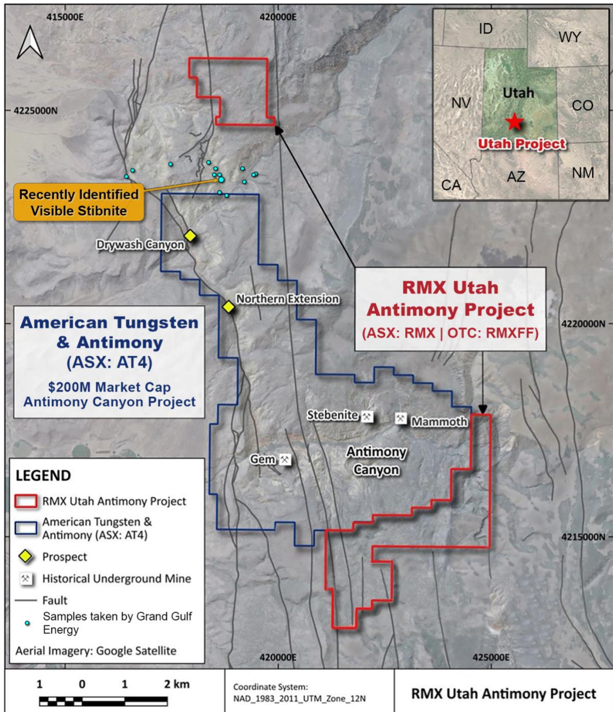
Figure 3: Location of Red Mountain's Utah Antimony Project relative to Americal Tungsten and Antimony Ltd's Antimony Canyon Project, with the new claim area highlighted. The locations of AT4's main focus areas - Antimony Canyon, and the Drywash Canyon and Northern Extension prospects, are also shown.
