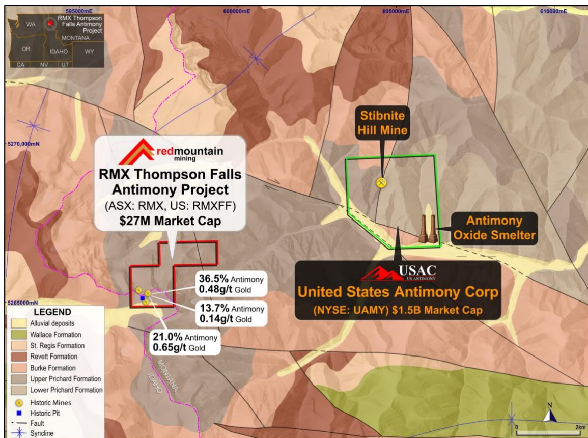
Figure 1: USGS geology of the area encompassing Red Mountain's Thompson Falls Antimony Project and UAMY's Thompson Falls Smelter and Stibnite Hill Antimony Mine. Red Mountain's observed locations of three historical underground mines and an open pit verified by first-pass exploration and highlights of initial rock chip sampling are also shown.
