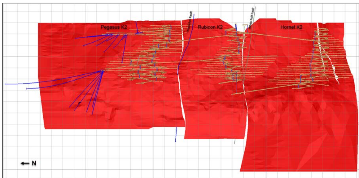
Figure 8 - Long section of RHP showing in-mine exploration drilling targeting Pegasus K2, Rubicon K2, and Hornet K2 during the December quarter.
