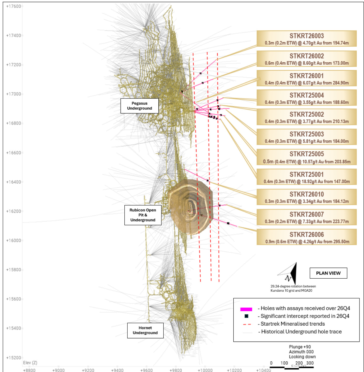
Figure 2 A Plan view of the assay results location returned from within the quarter for Star Trek. Image provided in K10 Mine Grid.
