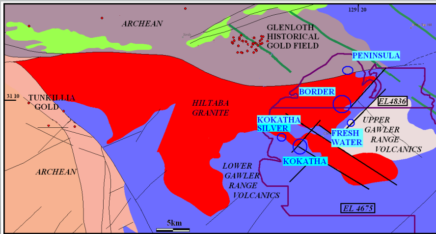
Gairdner Project, showing regional geology and prospects drilled in recently completed drill program
