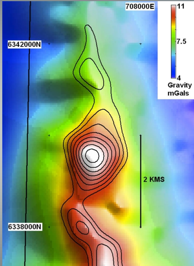
Nilginee, gravity contour image showing 0.5 Mgal intervals
