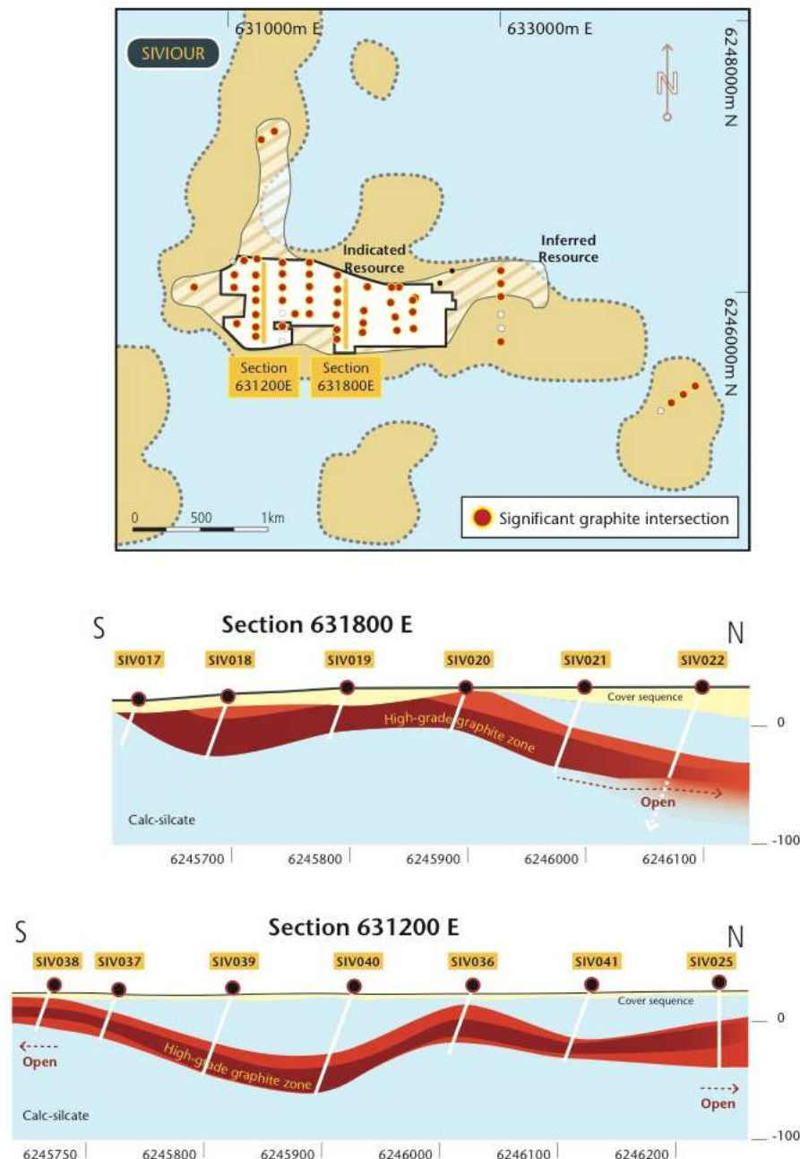
Figure 2. Siviour -- Plan view showing Indicated and Inferred Resources over electromagnetic conductive zones and cross-sections with TGC assay results (5%TGC cut-off in dark red and 3% TGC cut-off in light red) over north-south Sections 631200E and 631800E
