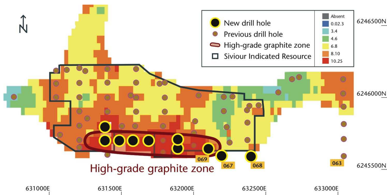
Figure 1. Siviour graphite deposit – average TGC% within the mineralised horizon of the Indicated Resource, showing new and previous drill holes in relation to high-grade graphite zone
