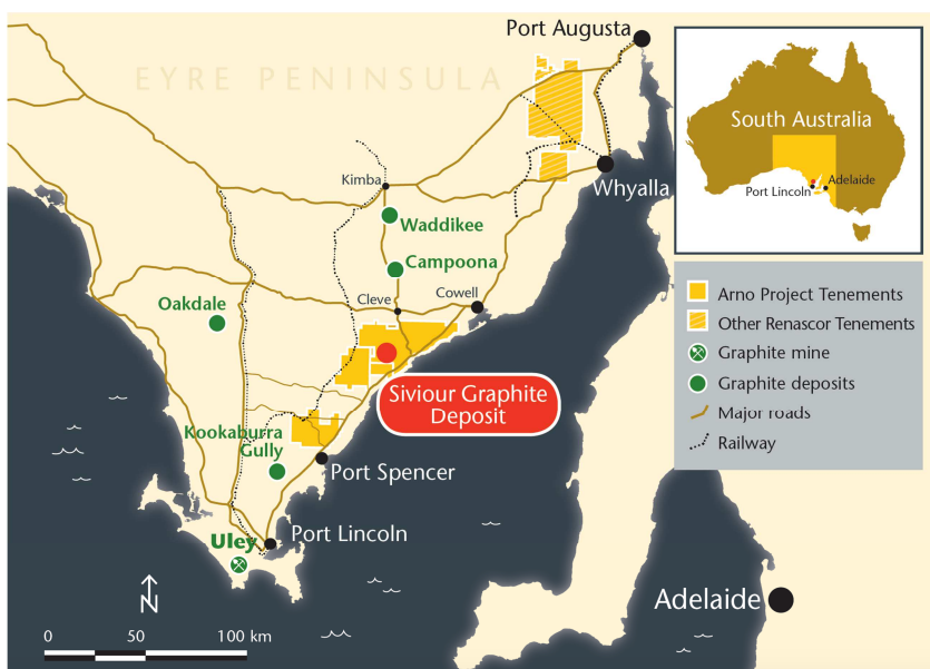
Figure 2. Siviour Graphite Deposit, showing location and significant nearby graphite deposits
