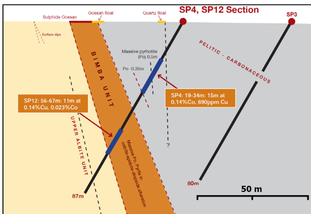
Figure 3. Shorts Dam historical drill section SP4-SP12-SP3 (Source: Esso, 1979)
