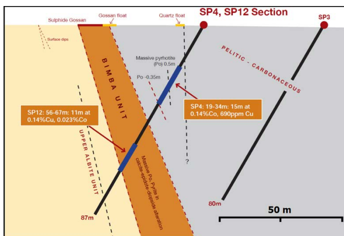
Figure 2. Shorts Dam historical drill section SP04-SP12-SP03 (Source: Esso, 1979)
