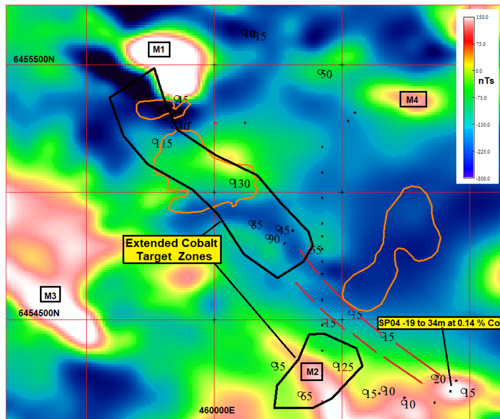
Figure 4. Shorts Dam – magnetic image and target anomalies M1 to M4
