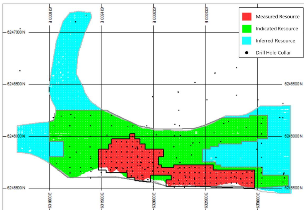
Figure 3. Plan view of the Siviour deposit showing the distribution of Resource classifications and drill hole locations
