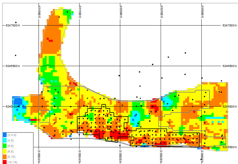
Figure 4. Plan view of the Siviour showing average TGC grade overlain with the outlines of Mineral Resource classifications and drill hole locations
