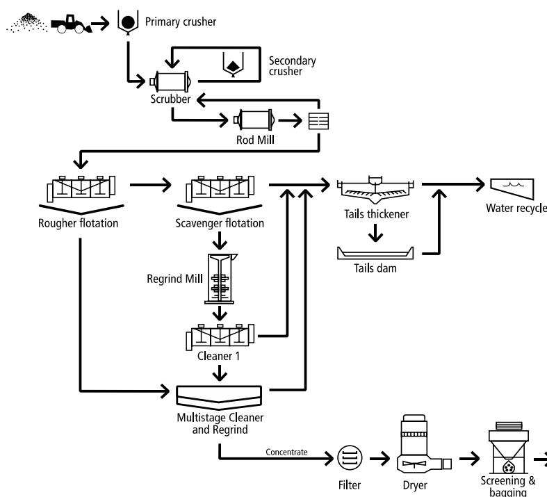
Figure 10. Process plant flowsheet
