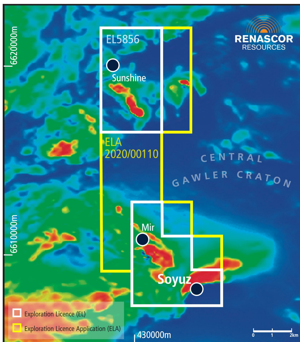
Figure 7. Renascor's Carnding Project, showing gold prospects over reduced to pole (RTP) magnetic image
