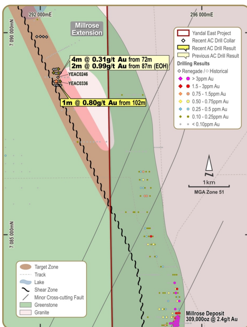
Figure 7. Location of drilling and significant intercepts at Millrose Extension
