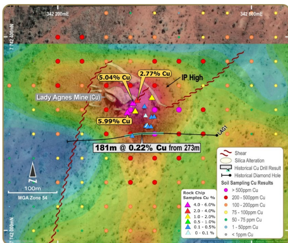
Figure 1: Lady Agnes Plan View – structures, soil results, rock chips, IP and LAG1
