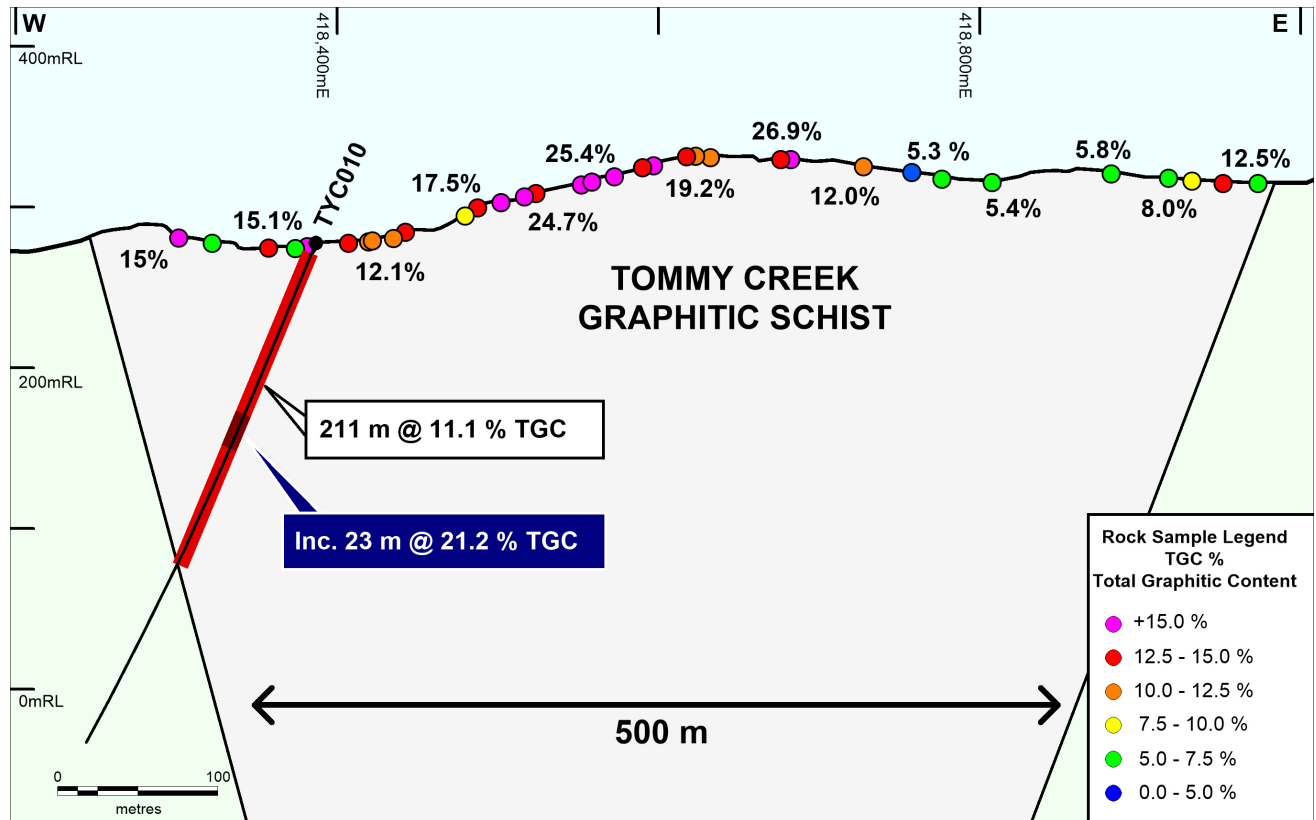
Figure 2: Cross section - Hole TYC010 looking north and showing Total Graphitic Content of surface rock samples.
