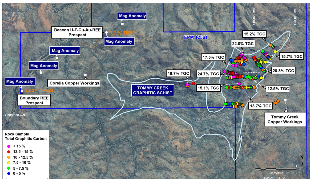
Figure 3: Tommy Creek prospect area of EPM1256.
