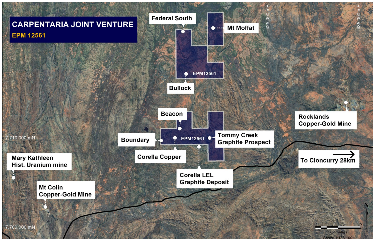
Figure 1. Location of EPM 12561 – Carpentaria Joint Venture, showing Tommy Creek Graphite prospect.
