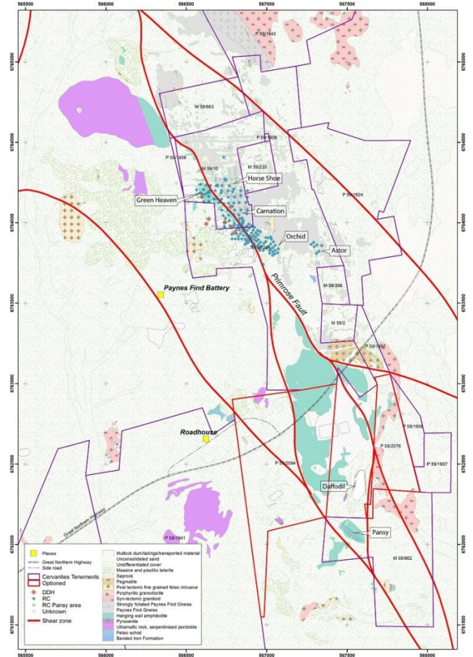
Fig 2. Project Tenements and Geology
