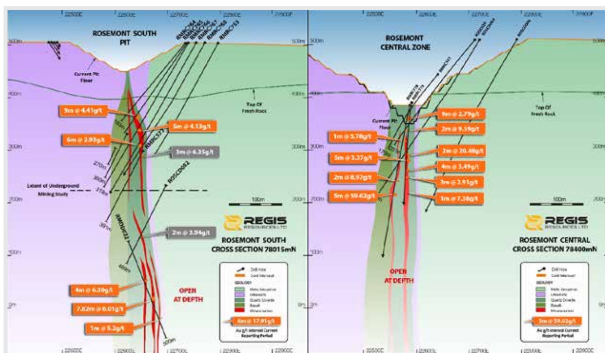
Section 78015mN showing high grade gold intercepts at Rosemont south, 200m below proposed UG development slope design. Cross Section 78400mN at Rosemont Central zone along strike and outside of current UG resource domains.
