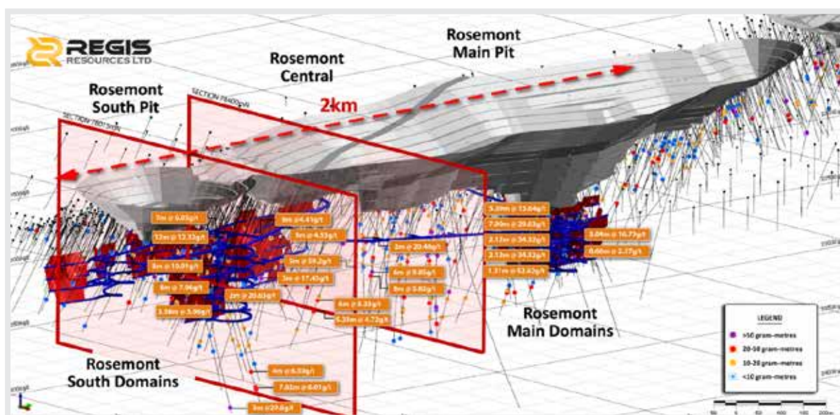
Oblique Long Section looking northwest shows final pit design and proposed UG mine design and stoping blocks.
