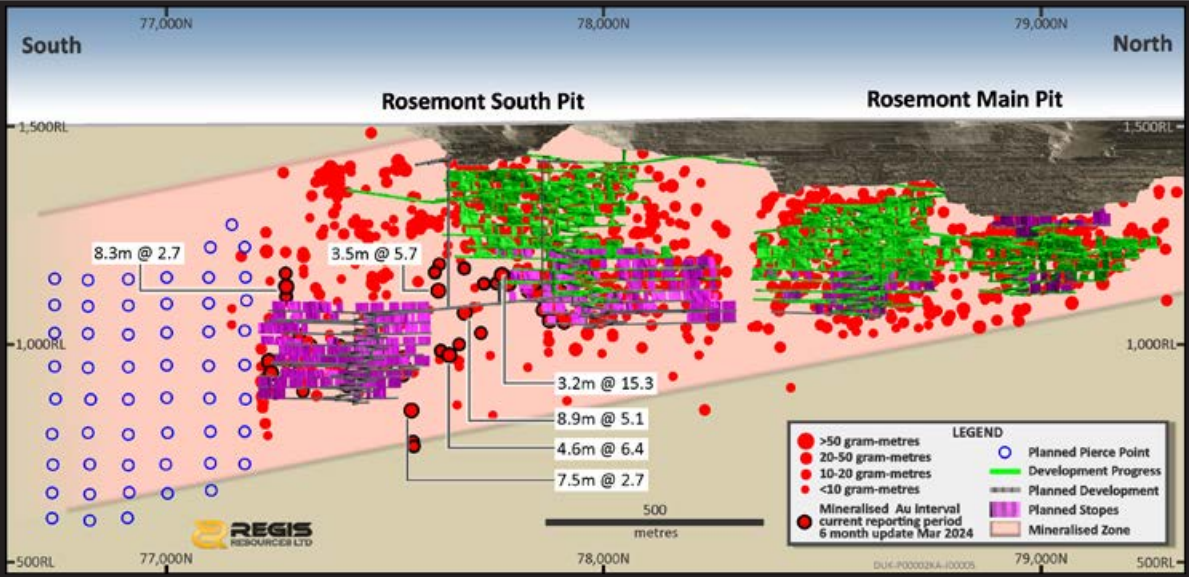
Figure 5: Rosemont long section showing new drill intersections outside the Stage 3 planned stopes and the planned pierce points down plunge.
