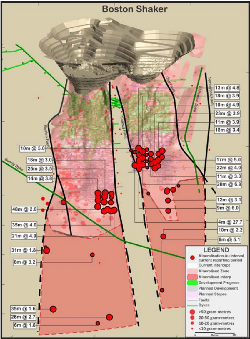
Figure 8: Boston Shaker long-section displaying gram metre pierce points and 0.3 g/t Au mineralisation zone and recent high-grade intersections.
