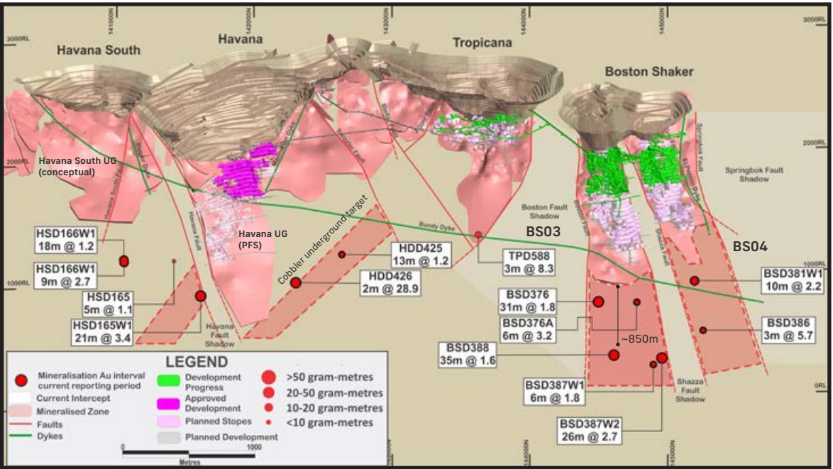
Figure 7: Tropicana oblique view of the mineralised corridor showing actual and conceptual open pit and underground production areas and the 0.3 g/t Au mineralised zones (pink).
