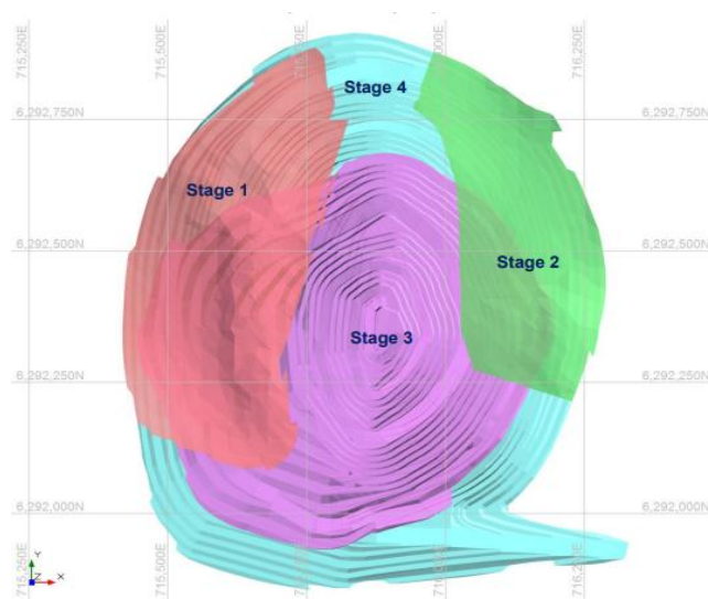
Figure 4: Pit Design Stages.
