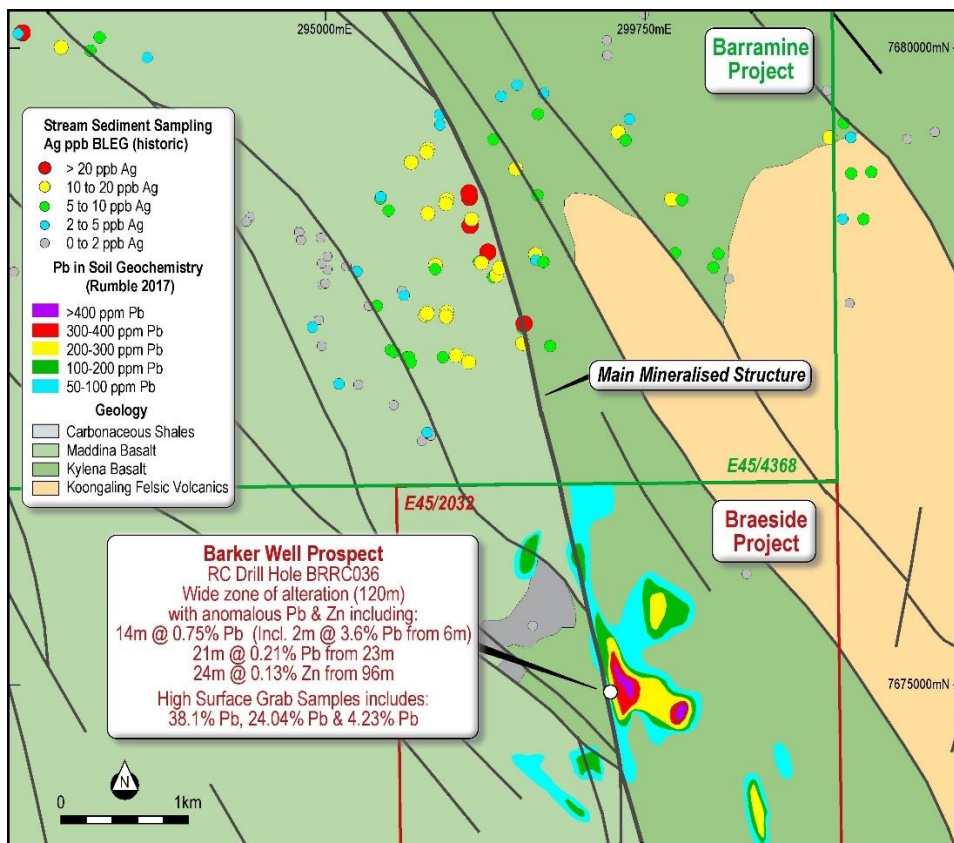
Image 3 – Southern Barramine Project – Extrapolation of Mineralised Structure from Braeside Project - Ag in Stream Sediment Anomalism
