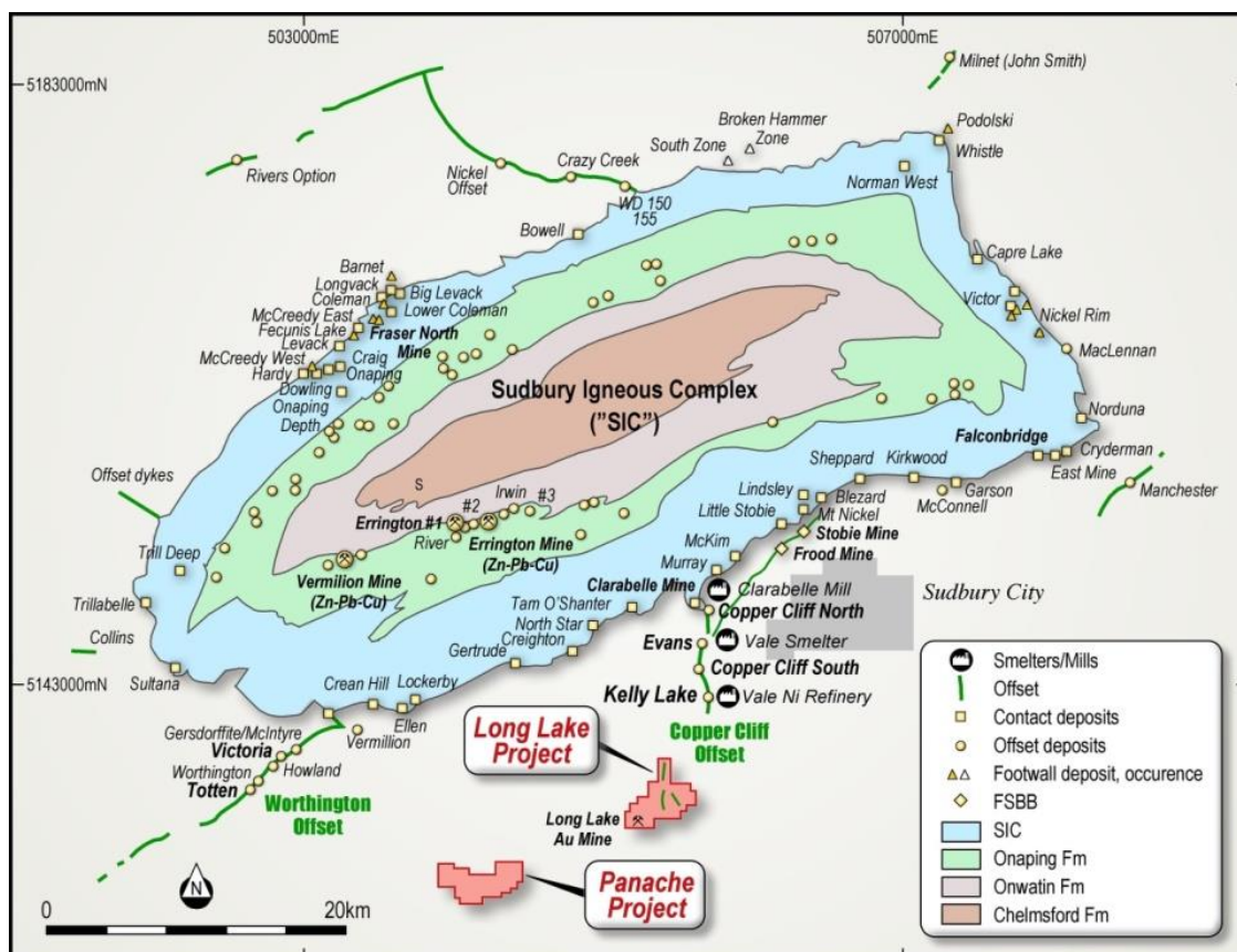
Image 1 – The location of the Long Lake Project, Copper Cliff Offset and Deposit Types of the Sudbury Basin.
