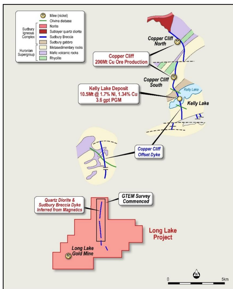
Image 2 – Inferred Copper Cliff Offset Dyke extension moved west – Location of Ground EM Survey
