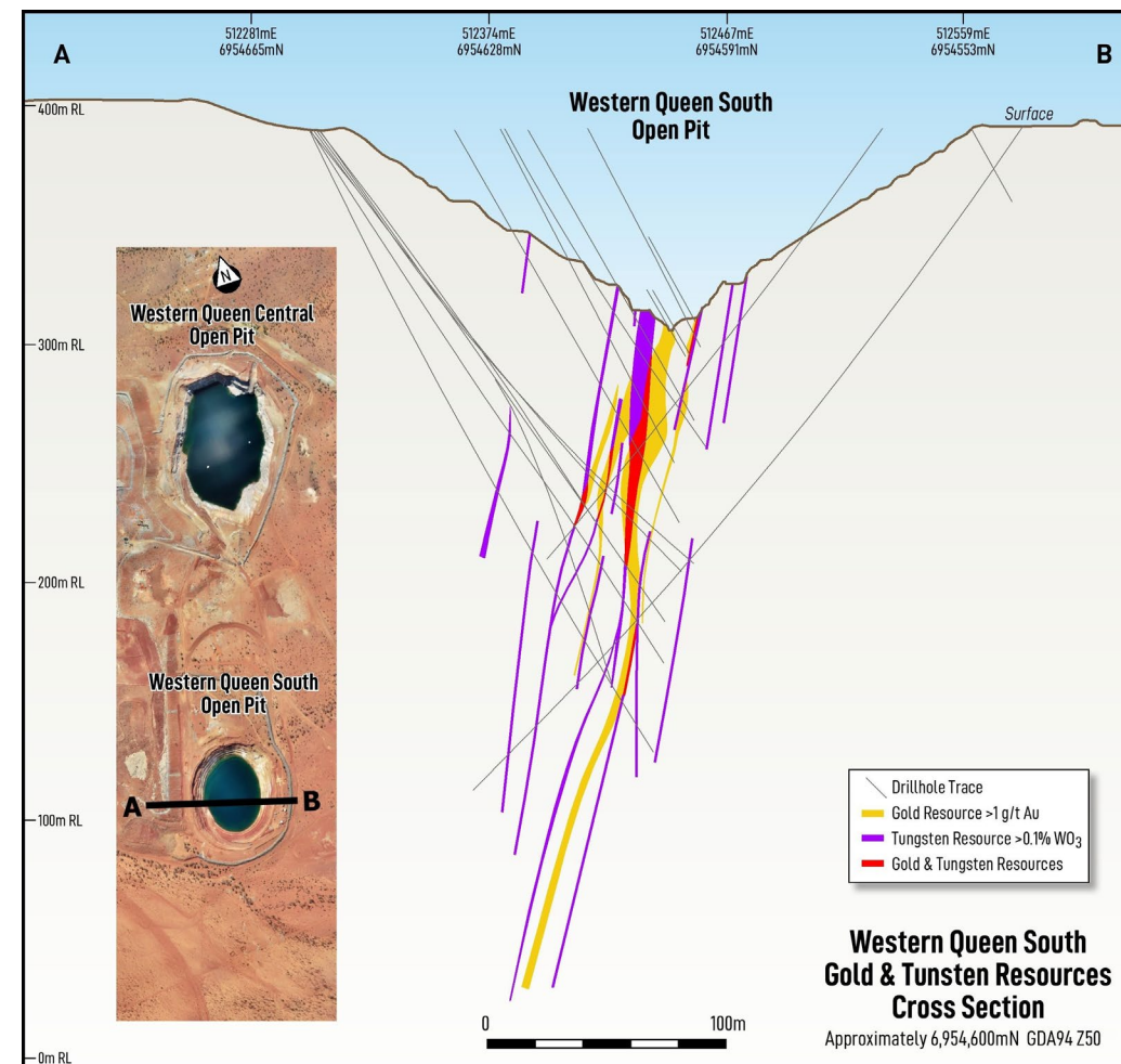
Cross section thru WQ South
