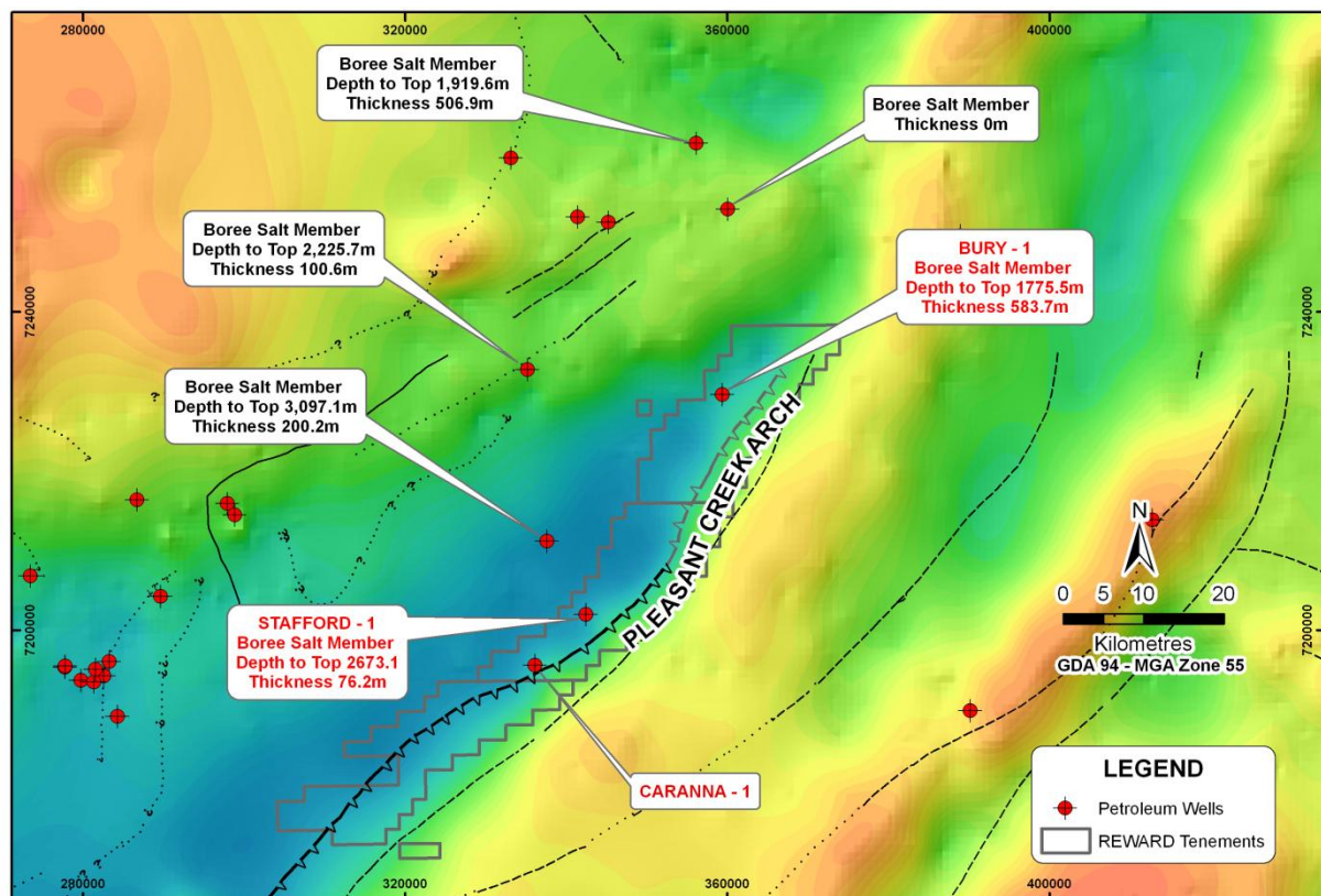
Figure 8 Gravity Image
