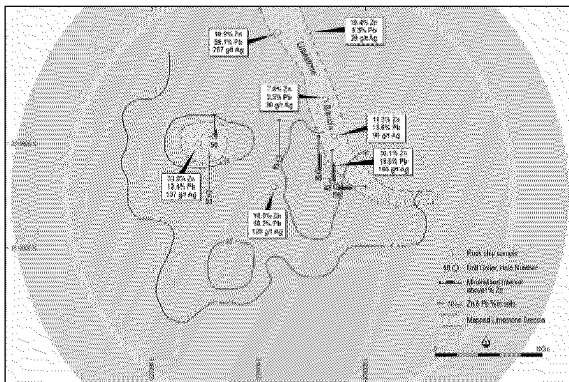
Figure 2: Pha Sod Drill, Soil Sample Contour and Rock Chip sampling plan
