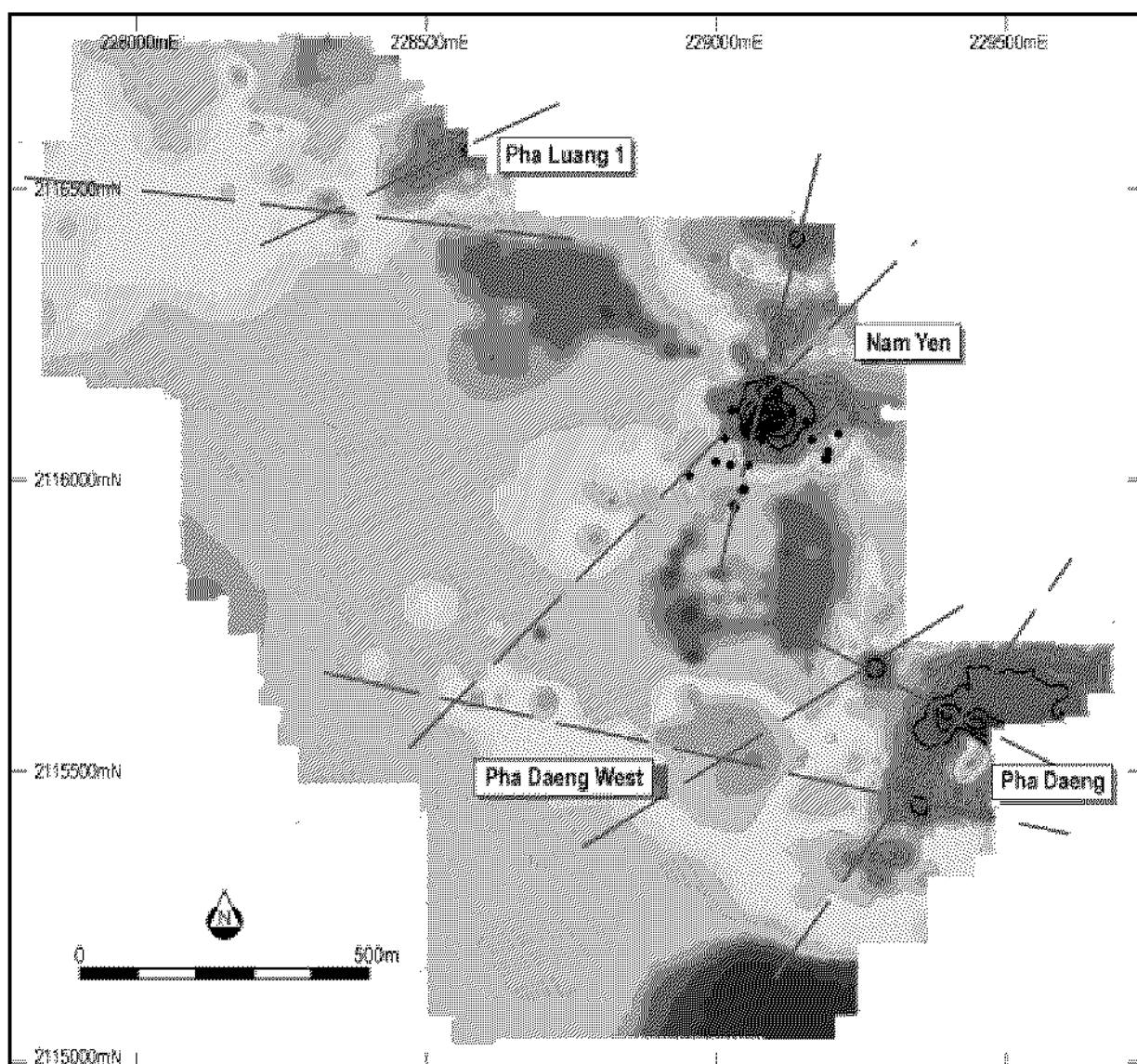
Figure 3: Pha Daeng area soil sampling plan showing possible mineralised structures
