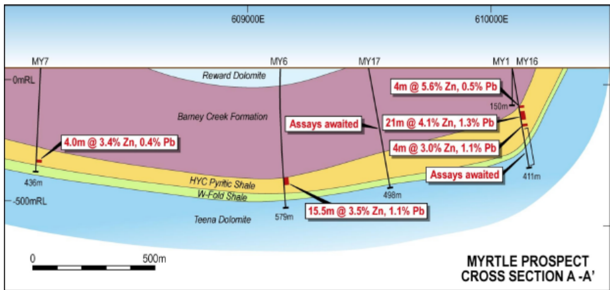
Figure 3: Myrtle Prospect Cross Section A-A' showing drill intercepts
