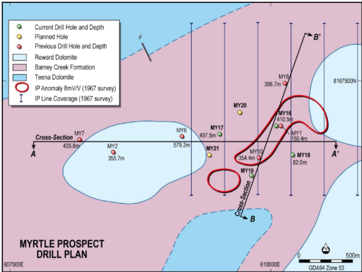
Figure 2: Myrtle Prospect Drill Plan, showing previously interpreted geology, IP anomaly location, and cross-section line A-A'
