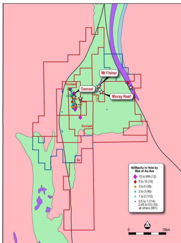
Figure 2: Mt Fisher Prospect Locations
