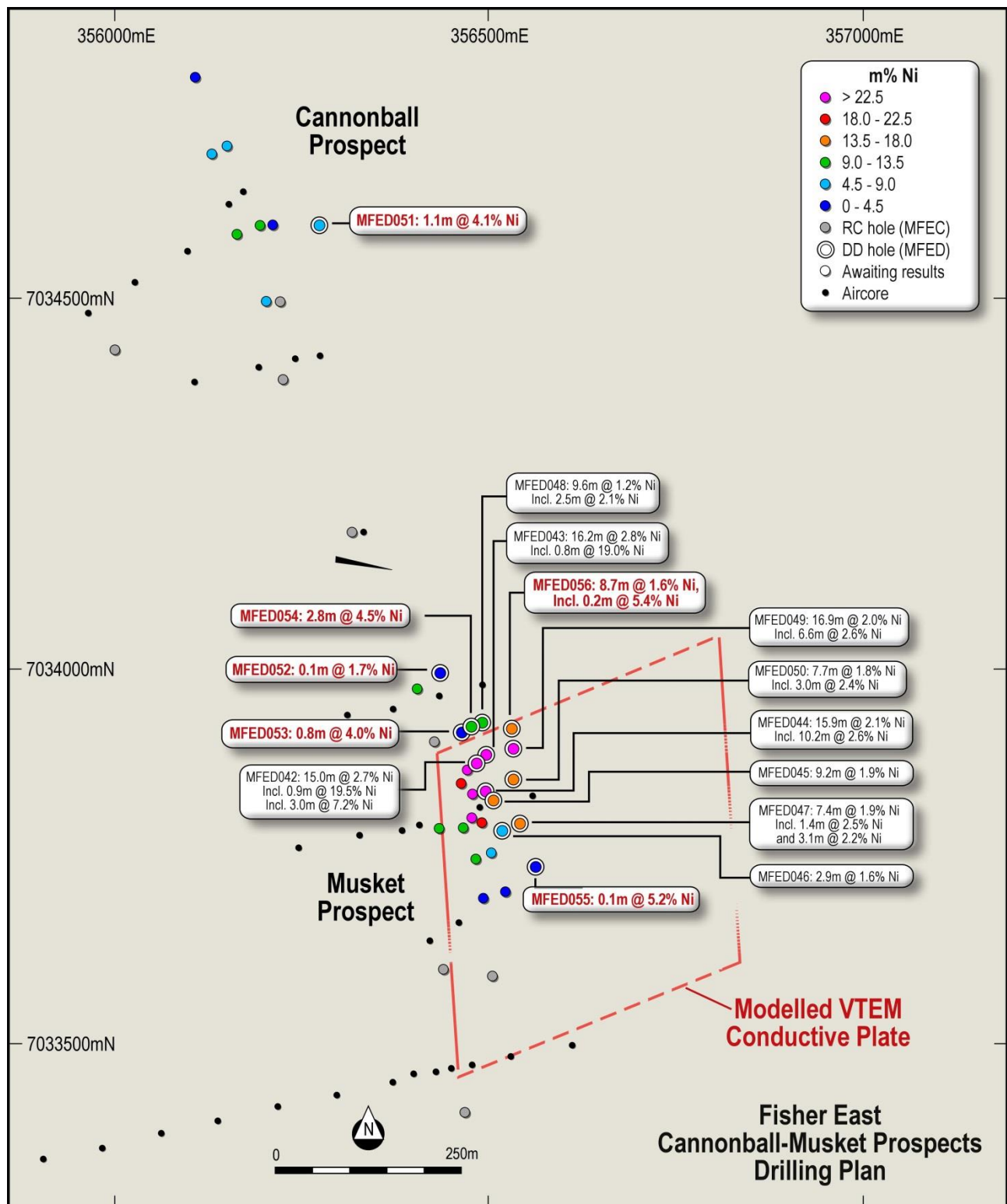
Figure 2: Cannonball – Musket Drill Plan
