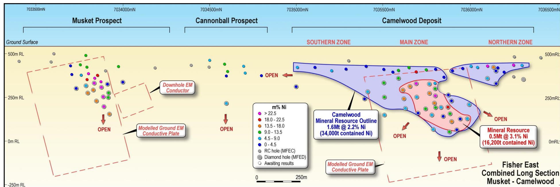
Figure 5: Camelwood – Musket Long Section
