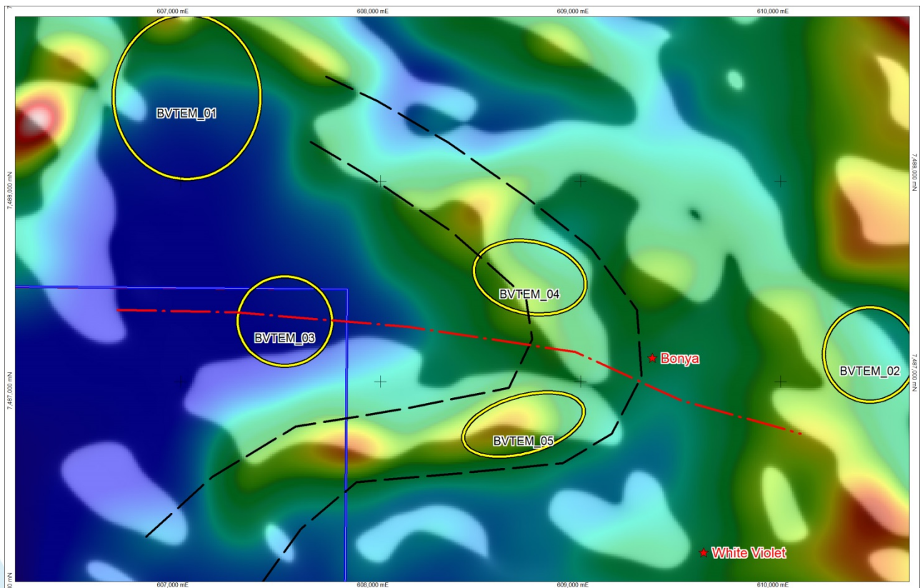
Figure 2: Bonyta magnetics showing interpreted geology (black lines) and fold axis (red line)
