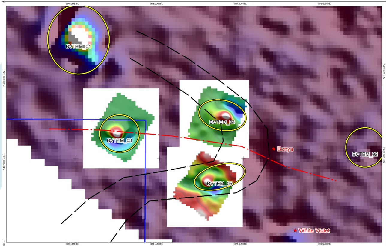
Figure 1: Bonyta VTEM and Ground EM showing interpreted geology (black lines) and fold axis (red line)
