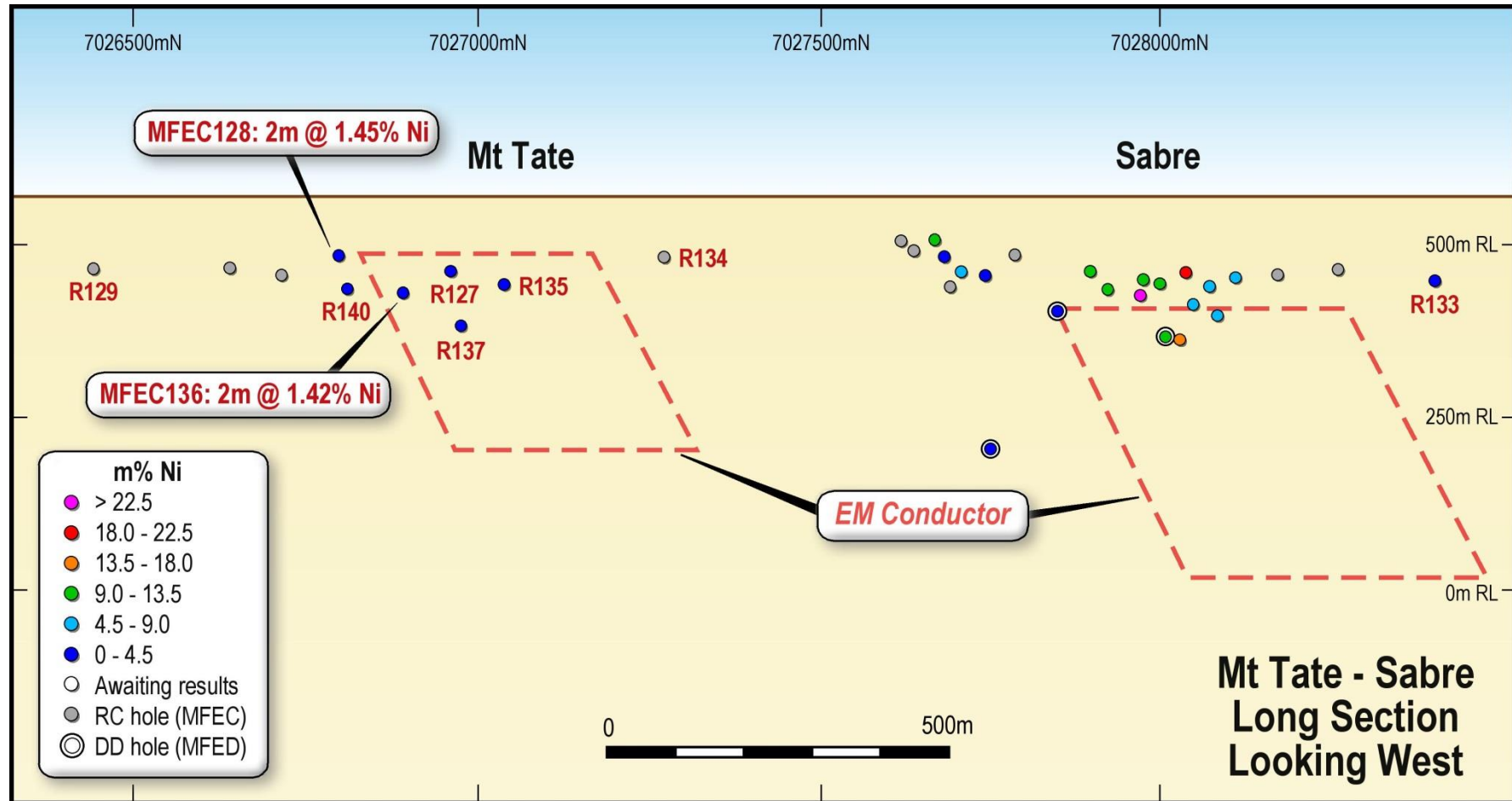
Figure 3: Mt Tate – Sabre Long Section
