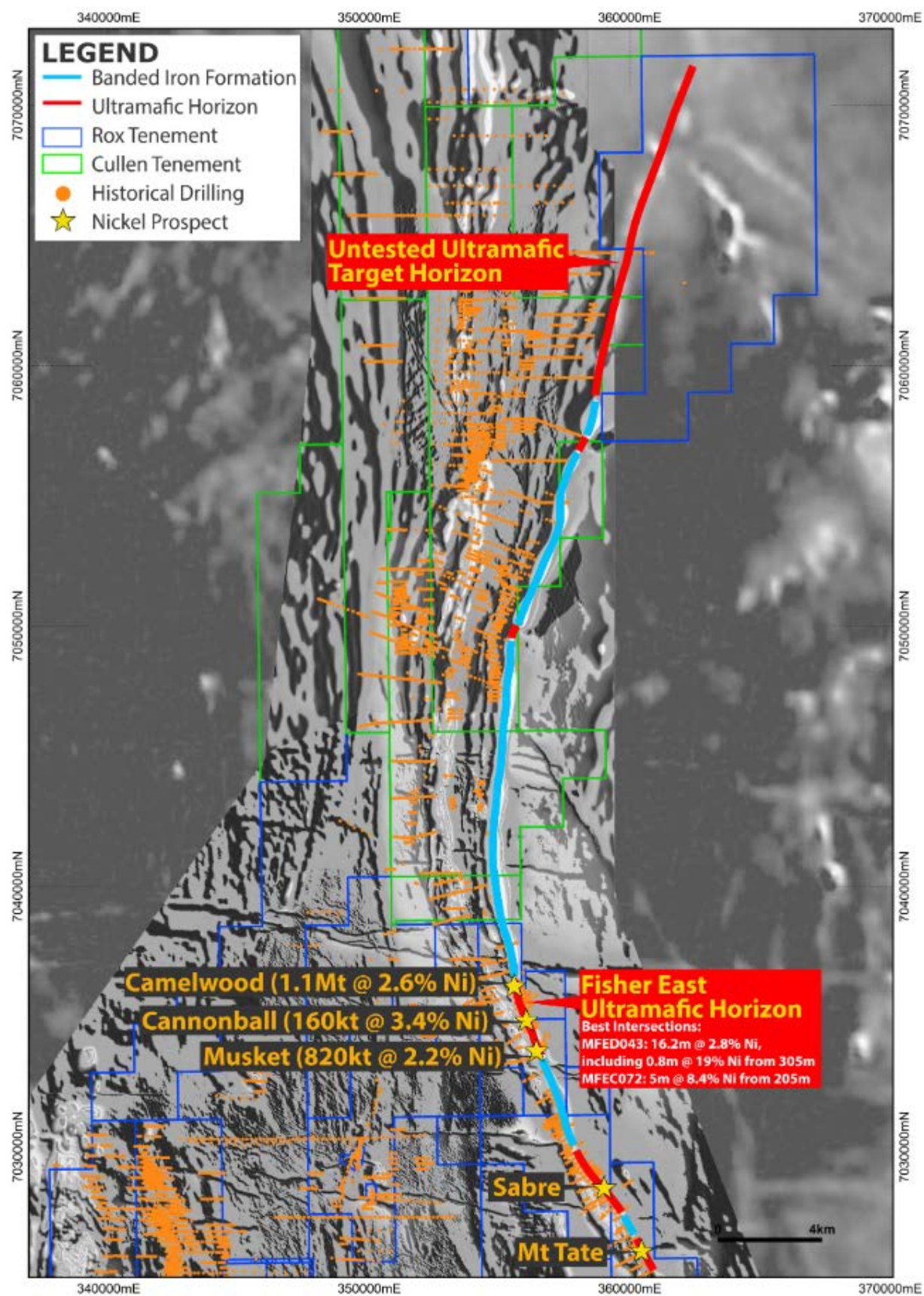
Figure 7 – Rox and Cullen Tenure on Magnetics. Nickel Prospective Horizon Highlighted
