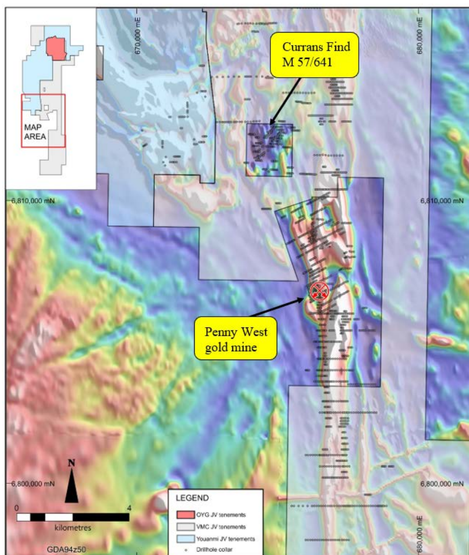
Figure 6 - Gold Mineralisation and Demagnetised Horizons running NNW through the belt to Currans Find Prospect
