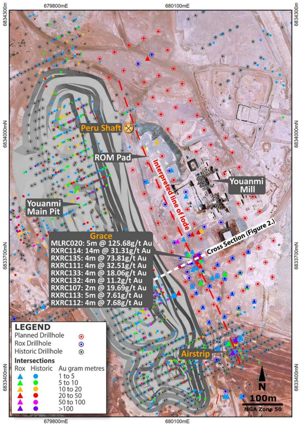
Figure 3 - Aerial photo with drill collars & intersections overlaid
