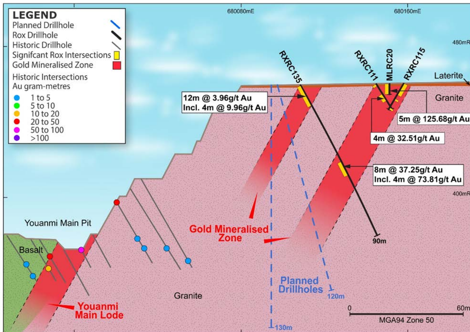
Figure 4 – Cross Section through Main Pit and Grace Prospect showing depth extension and new HW mineralisation
