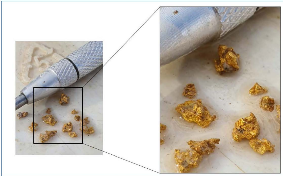
Figure 5 - Visible Gold Encountered in MLRC020
