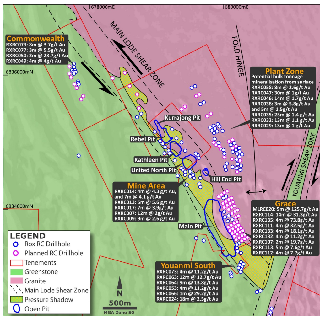
Figure 2 –Youanmi Pits Overlain on Geology with RC Drill Collars
