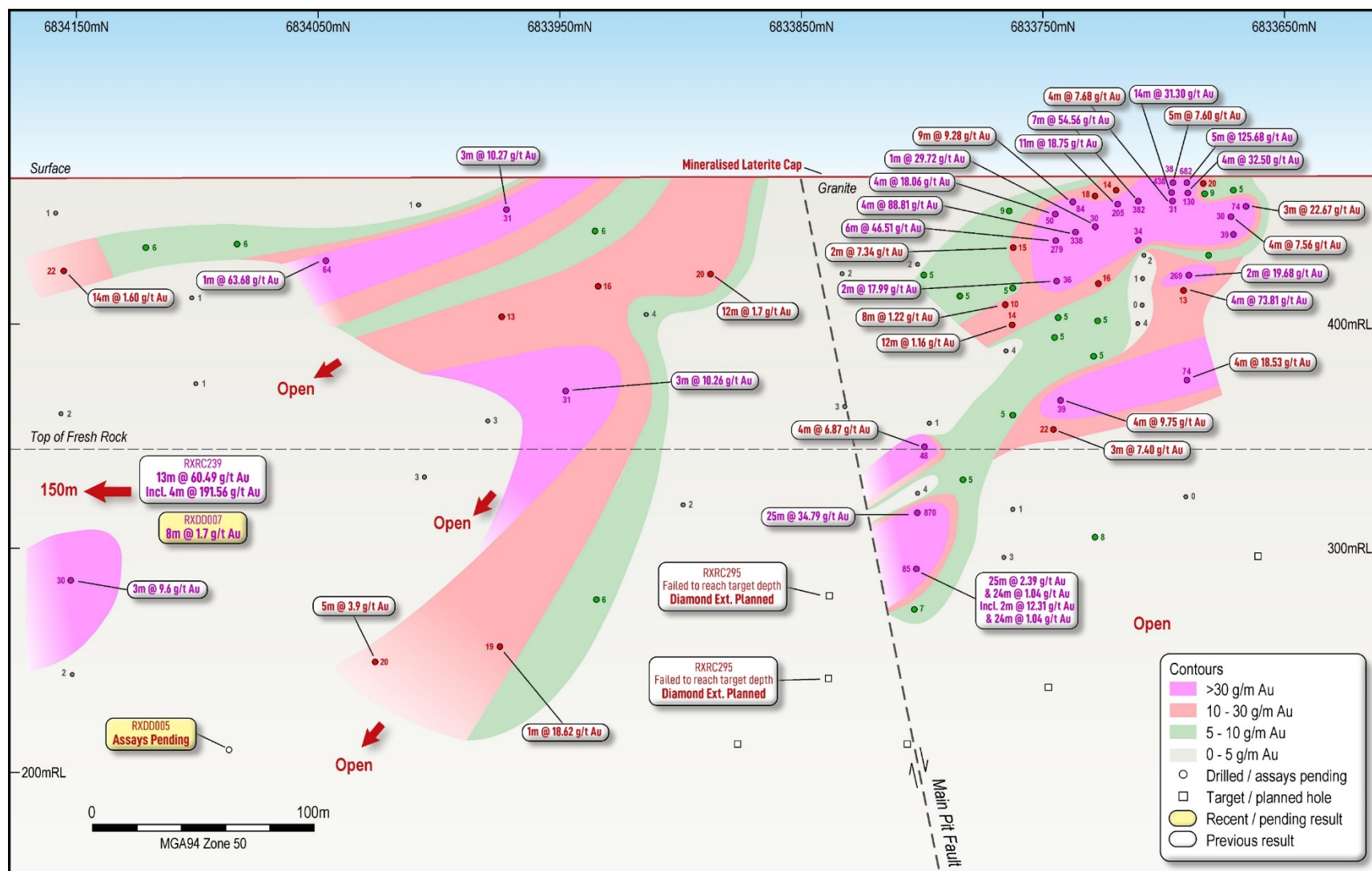
Figure 1 - Grace Prospect Long Section
