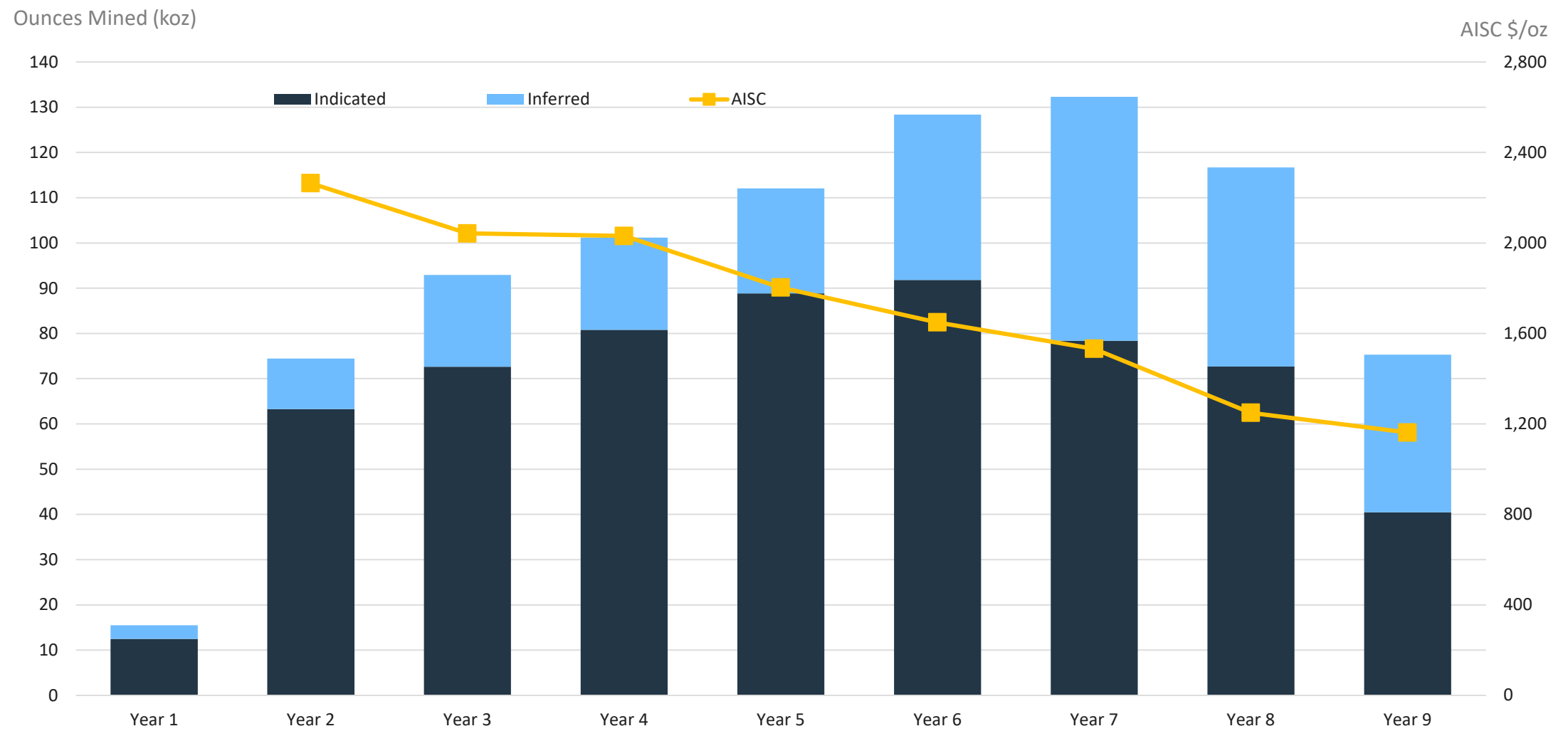
Life of Mine Ounces Mined and AISC
