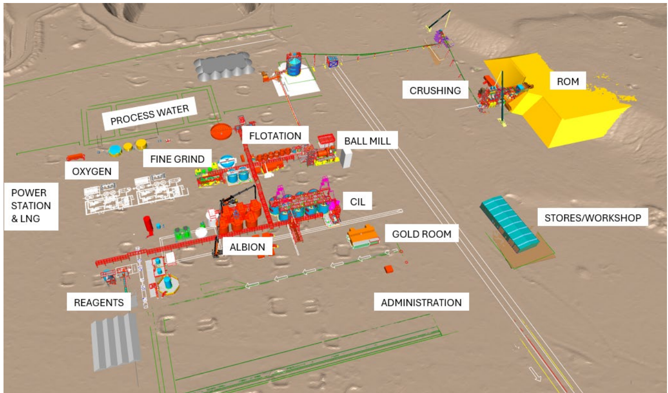
Figure 5 – Process plant working layout
